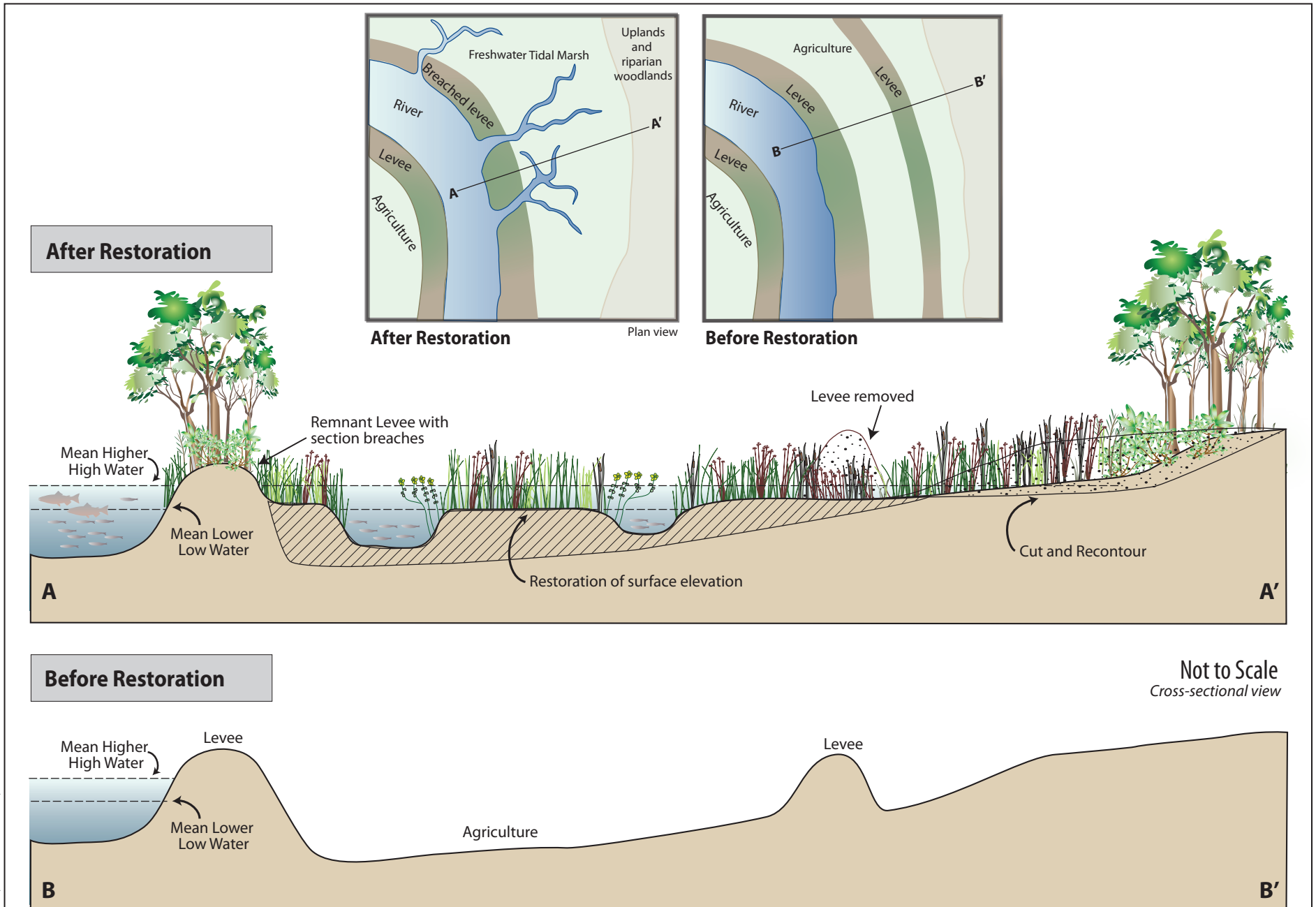
Figure 5-1 Conceptual Design for Restored Tidal Freshwater Emergent Wetland
