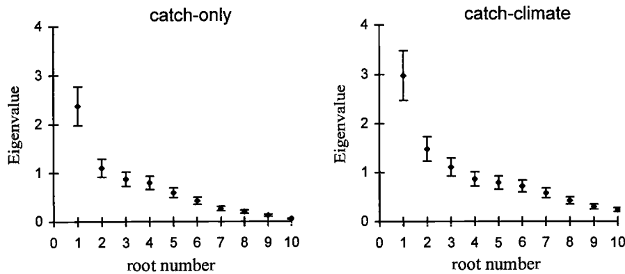
Figure 4 shows Eigenvalue scree plots from the catch-only and catch-climate principal component analyses. Error bars were computed by the formula of North et al. (1982).
