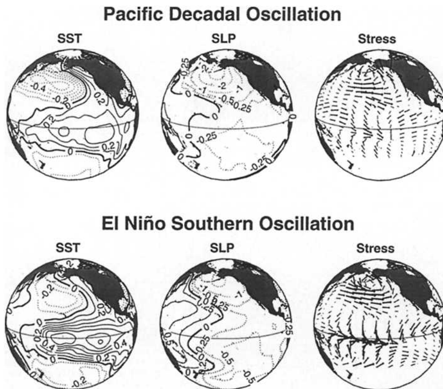
Figure 2 illustrates a comparison of anomalous climate conditions associated with the positive phases of the Pacific Decadal Oscillation (PDO) and El Niño Southern Oscillation (ENSO). The values show C for sea surface temperature (SST), millibars for sea level pressure (SLP) and direction and intensity of surface wind stress. The longest wind vectors represent a stress of 10 \text{ m}^2/\text{s}^2 . Actual anomaly values for a given year associated with the PDO and ENSO are computed by multiplying the climate anomaly with the associated temporal index (Figure 3). Adapted from Mantua et al. (1997).
