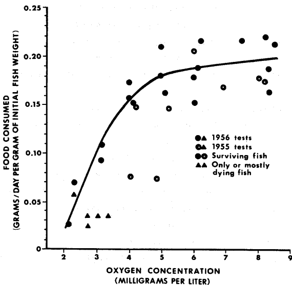
Figure 22—Grams of food (beach hoppers) consumed by frequently fed age-class 0 salmon per day per gram of initial weight of the fish, in relation to dissolved oxygen concentration. The curve has been fitted to only the 1956 data (from Herrmann et al. 1962).
