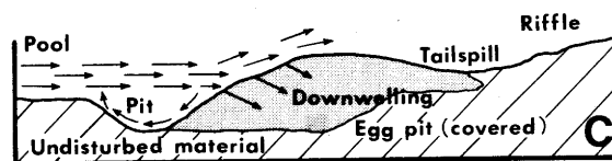
Figure 3—Longitudinal sections of spawning areas (from Reiser and Wesche 1977): A. Convexity of the substrate at pool-riffle interchange induces downwelling of water into the gravel. Area likely to be used for spawning is marked with an X. B. Redd construction results in negligible currents in the pit (facilitating egg deposition) and increased currents over and through (downwelling) the tailspill. C. Egg-covering activity results in the formation of a second pit which may also be used for spawning, as well as covering the eggs in the first pit. Increased permeability and the convexity of the tailspill substrate induces downwelling of water into the gravel, creating a current past eggs, bringing oxygen to them and removing metabolic wastes.
