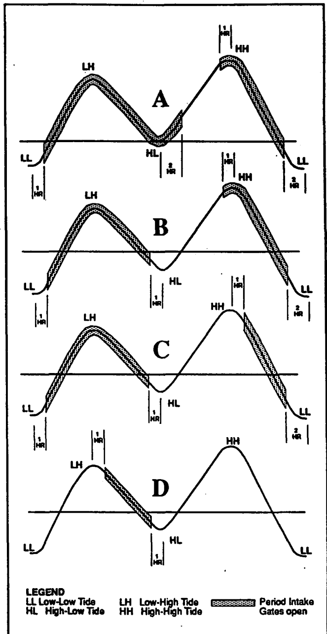
Figure 15 OPERATION PATTERNS OF CLIFTON COURT FOREBAY RADIAL GATES
