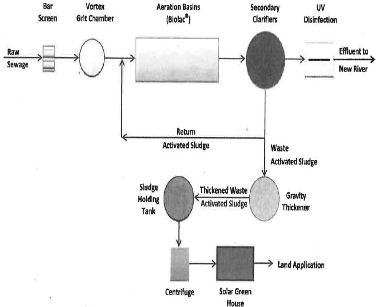
CITY OF BRAWLEY WASTEWATER TREATMENT PLANT FLOW DIAGRAM
