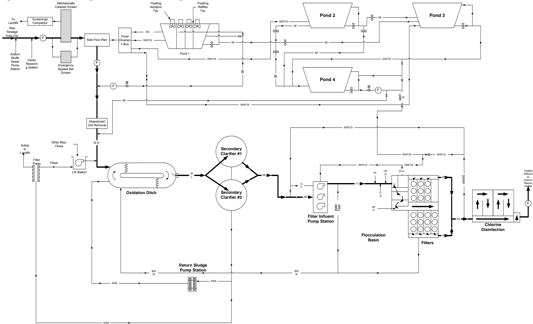
Figure C-1. Existing Process Flow Diagram
