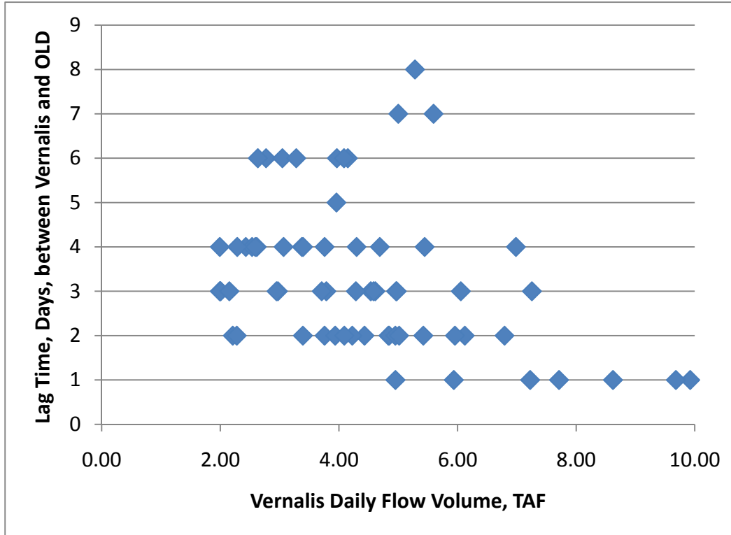
Figure 12: Lag Time between Vernalis and Old River near Tracy as a function of Vernalis flow
