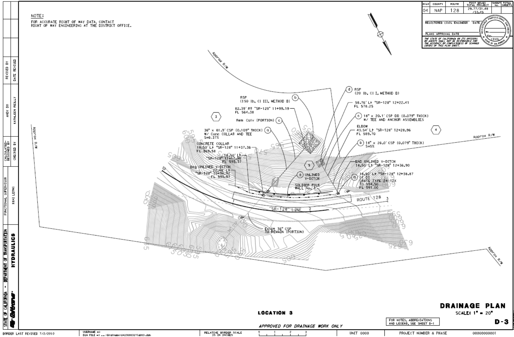
Figure 1: Drainage Plan
