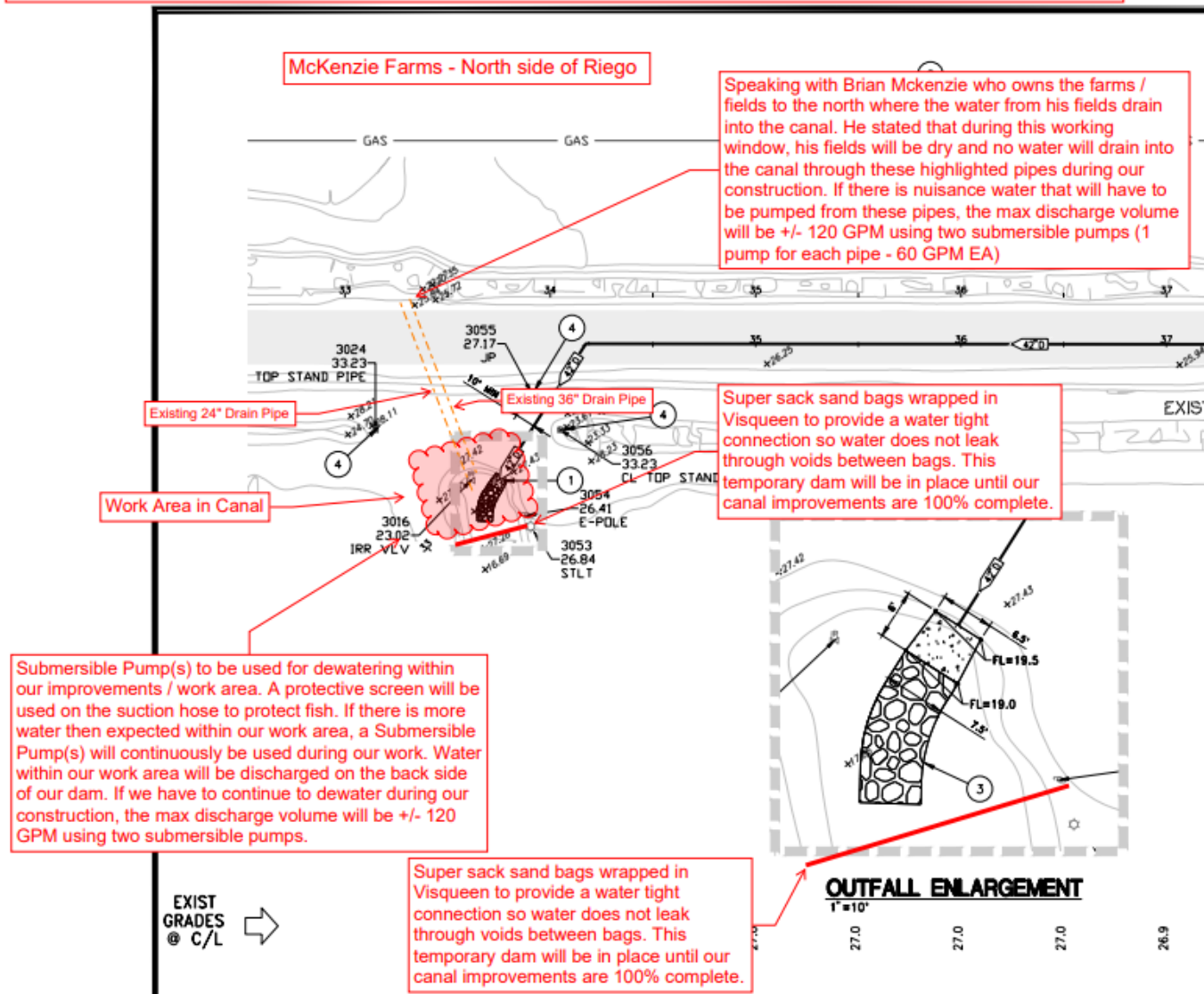
Outfall Dewatering Plan for Working Window: September 16th - November 1st
