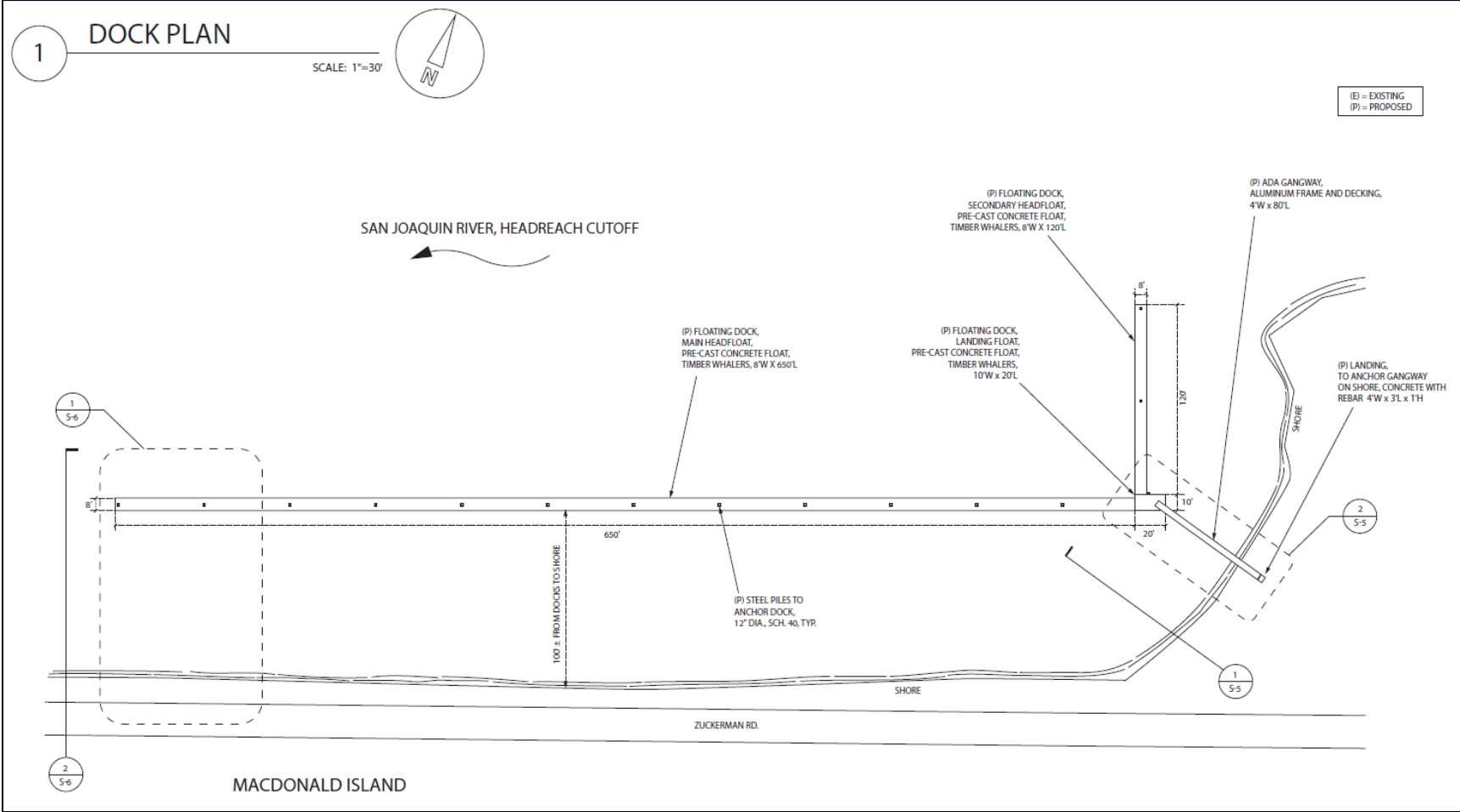
Figure 2: Project Plans
