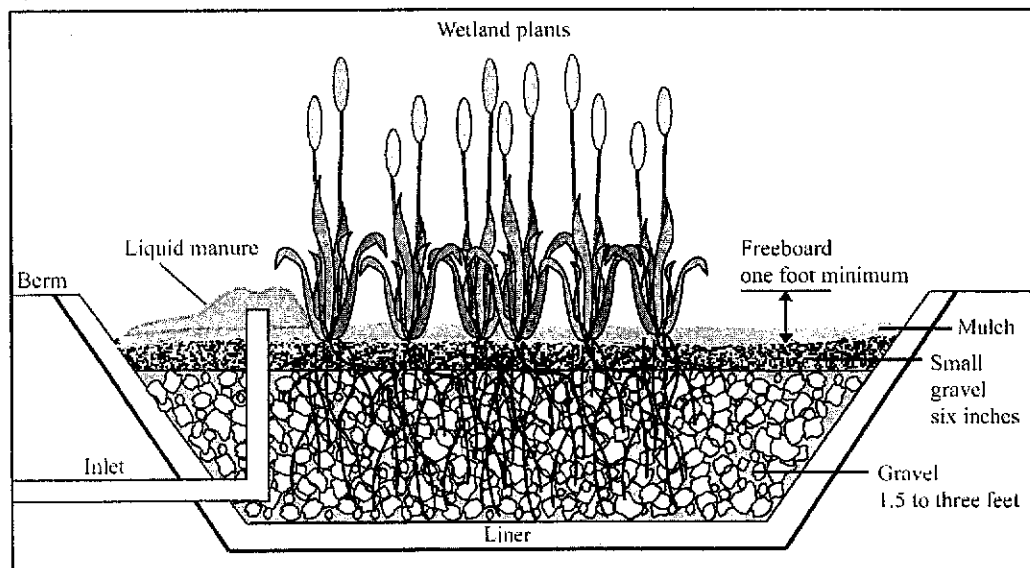
Figure 8.5: Diagram of subsurface flow wetland (C. White, 2004).
