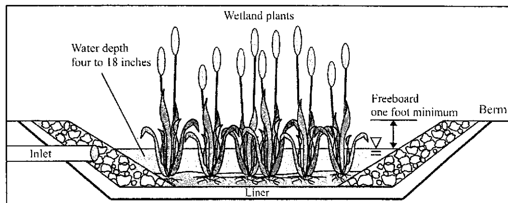
Figure 8.3: Diagram of open wetland (C. White, 2004).
