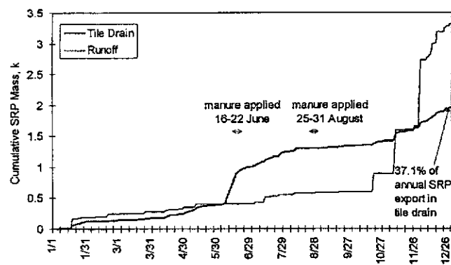
Figure 5—Cumulative annual soluble reactive phosphorus delivery from the tile drain and surface runoff during 1996 at the Catskills site.
