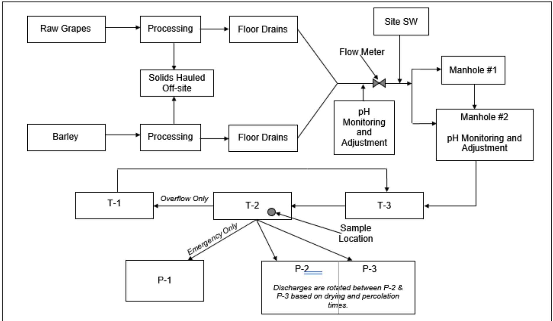
WASTEWATER FLOW SCHEMATIC CALIFORNIA CONCENTRATES COMPANY SAN JOAQUIN COUNTY
