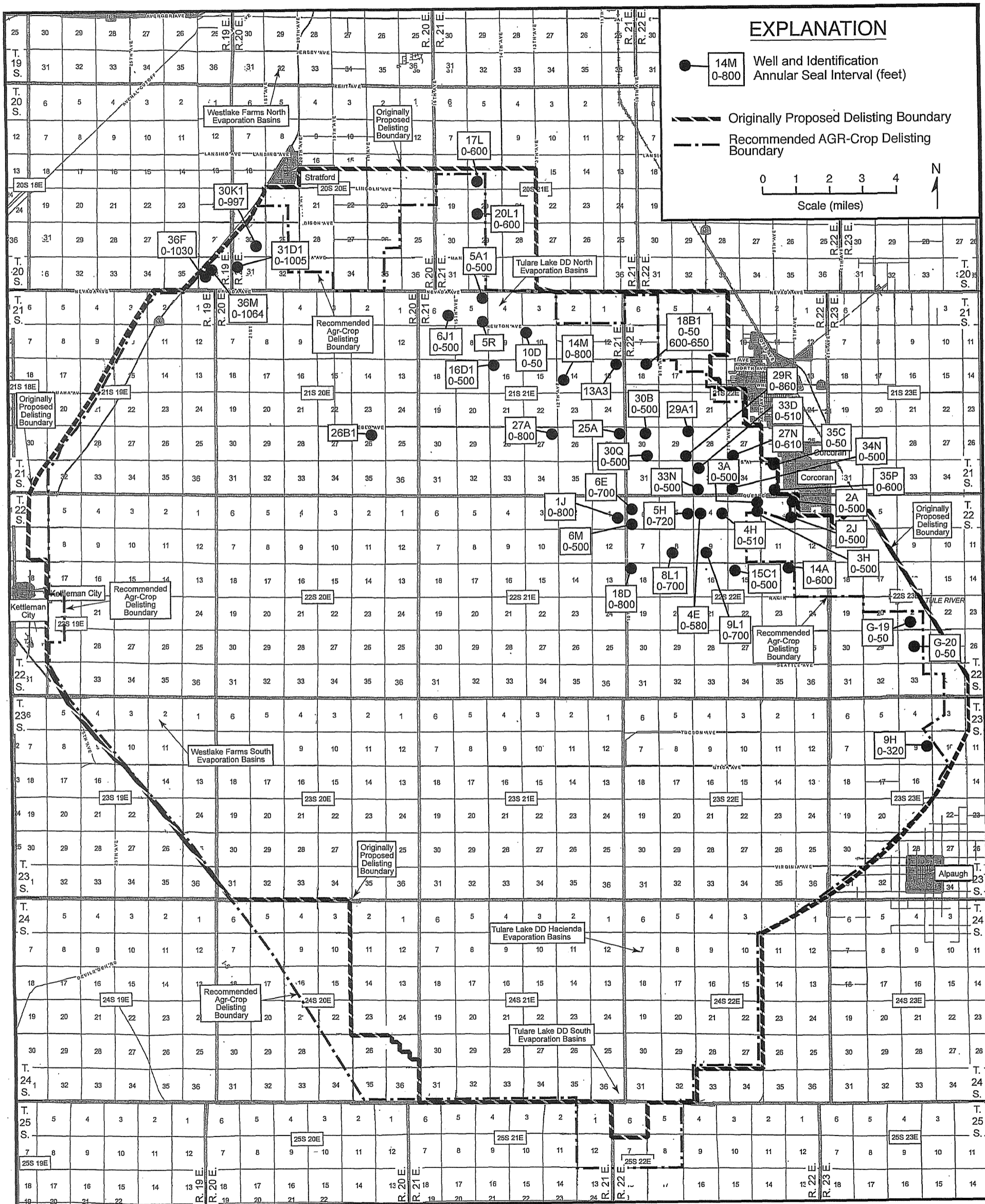
FIGURE B - ANNULAR SEAL INTERVALS FOR ACTIVE IRRIGATION WELLS AND REVISED RECOMMENDED AGR-CROP DELISTING BOUNDARIES
