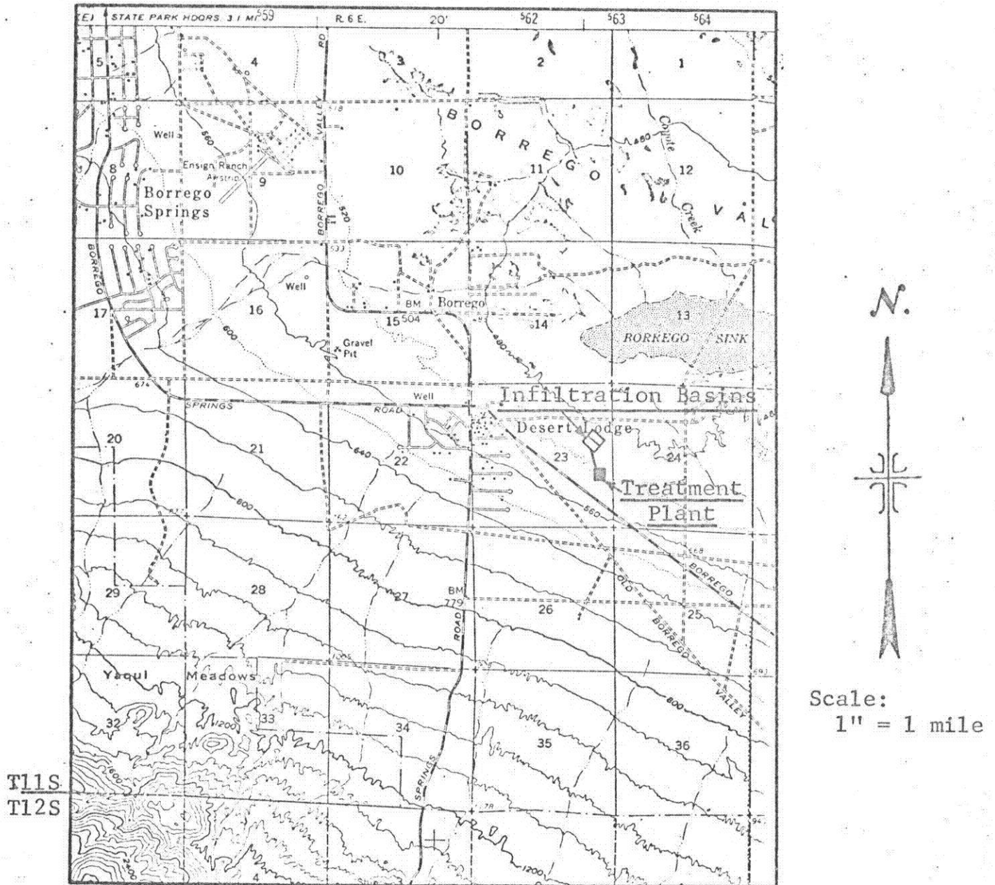
SITE MAP BORREGO WATER DISTRICT Borrego Springs - San Diego County Location of Discharge: NE \frac{1}{4} of Section 23, T11S, R6E, SBB&M USGS Borrego 15 min. Topographic Map
