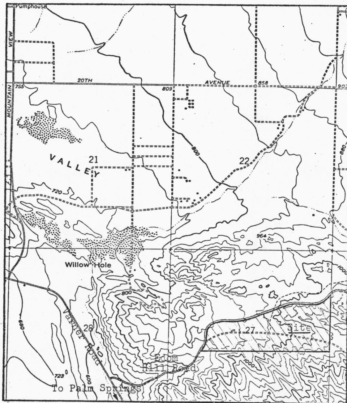
SITE MAP VISTA RV AND AQUATIC PARK Northeast of Palm Springs - Riverside County The Center Portion of Section 27, T3S, R5E, SBB&M USGS Seven Palms Valley 7.5 min. Topographic Map
