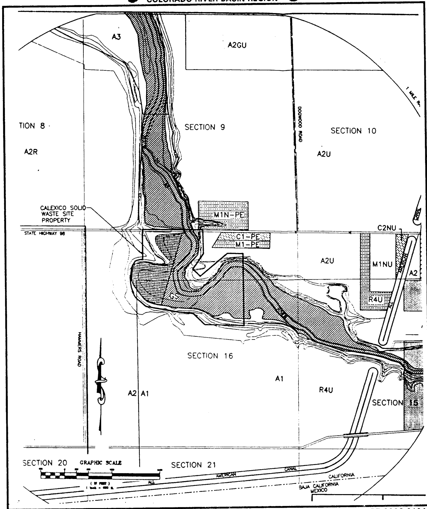
ATTACHMENT B SITE MAP COUNTY OF IMPERIAL, OWNER/OPERATOR CALEXICO CLASS III MUNICIPAL SOLID WASTE MANAGEMENT FACILITY Calexico - Imperial County
