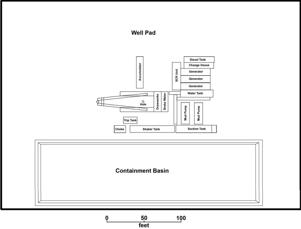
Figure 1: Typical Well Pad Layout Diagram
