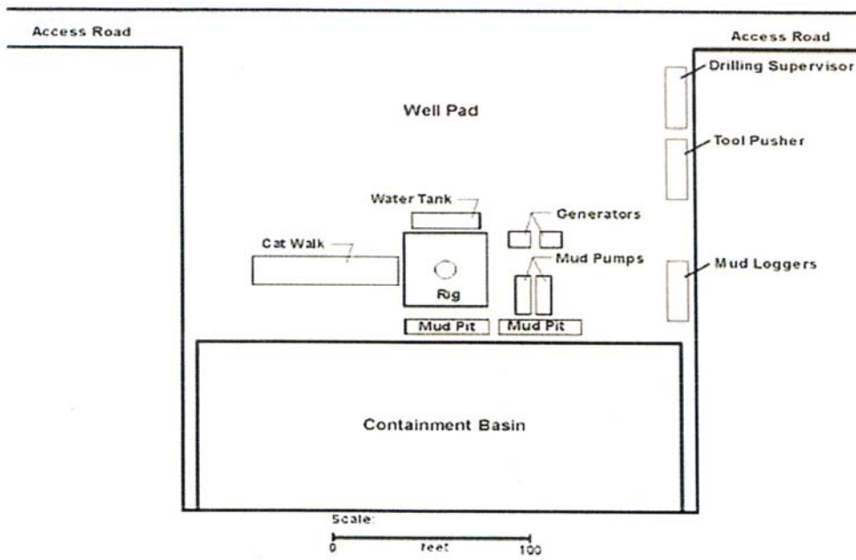
Figure 4: Typical Well Pad Layout Diagram
