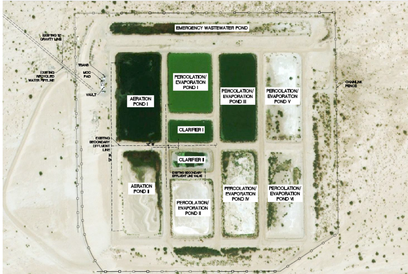
Figure 2. Site Plan
