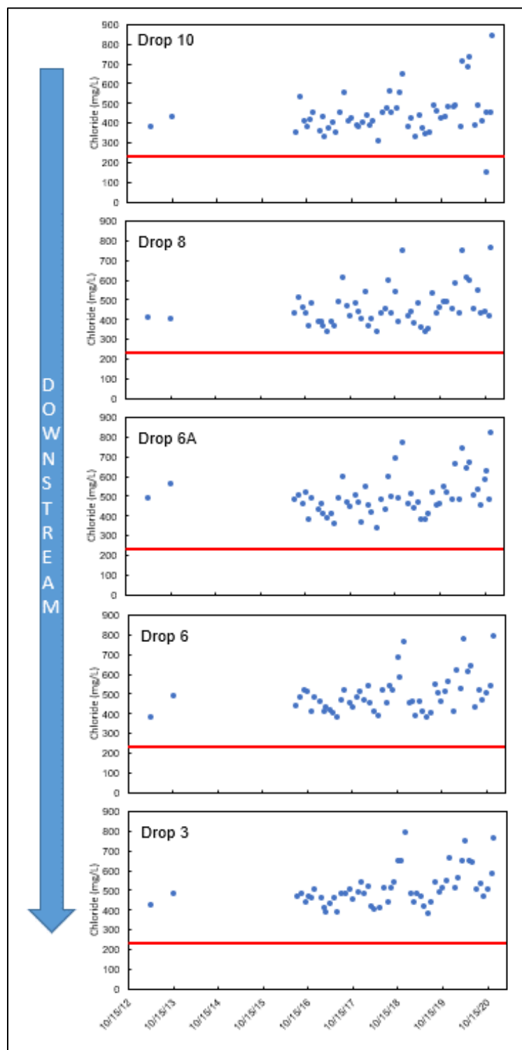
Figure 8: Chloride Concentrations at Multiple Sites on Alamo River
