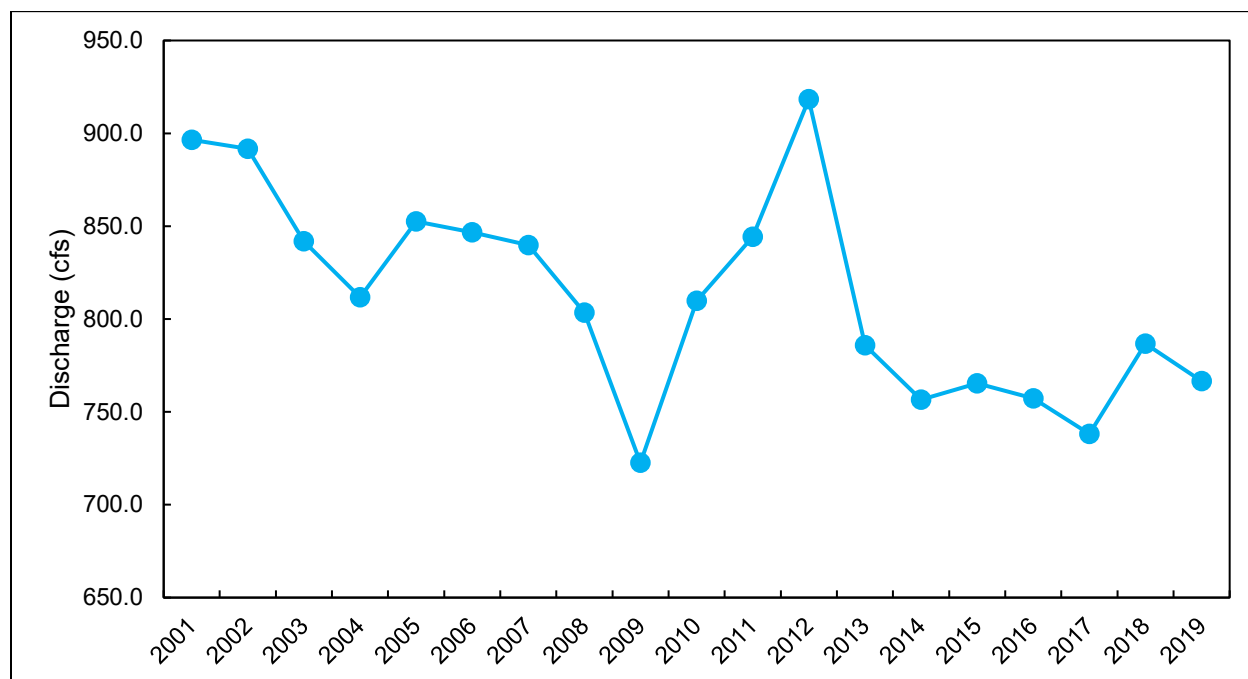
Figure 2: Annual Discharge Rates from Alamo River at Niland (USGS Natl Water Info System Data, Site No. 10254730)
