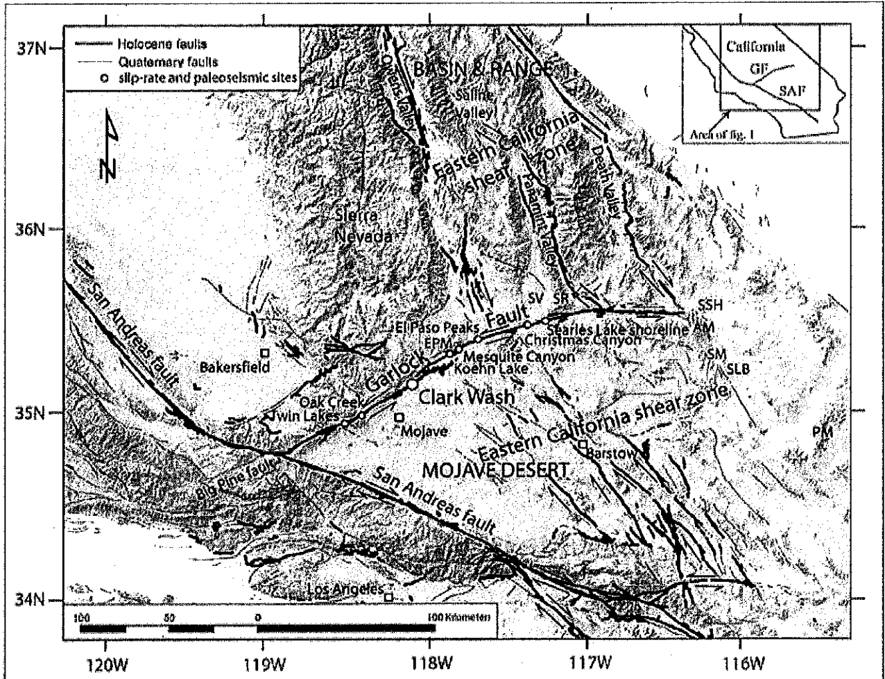
Figure 1: Location of the Clark wash site (large white circle) as well as other slip-rate and paleoseismic sites (small white circles) along the Garlock fault. AM, Avawatz Mountains; EPM, El Paso Mountains; PM, Providence Mountains; SLB, Soda Lake Basin; SM, Soda Mountains; SR, Slate Range; SSH, Salt Spring Hills; SV, Searles Valley.
