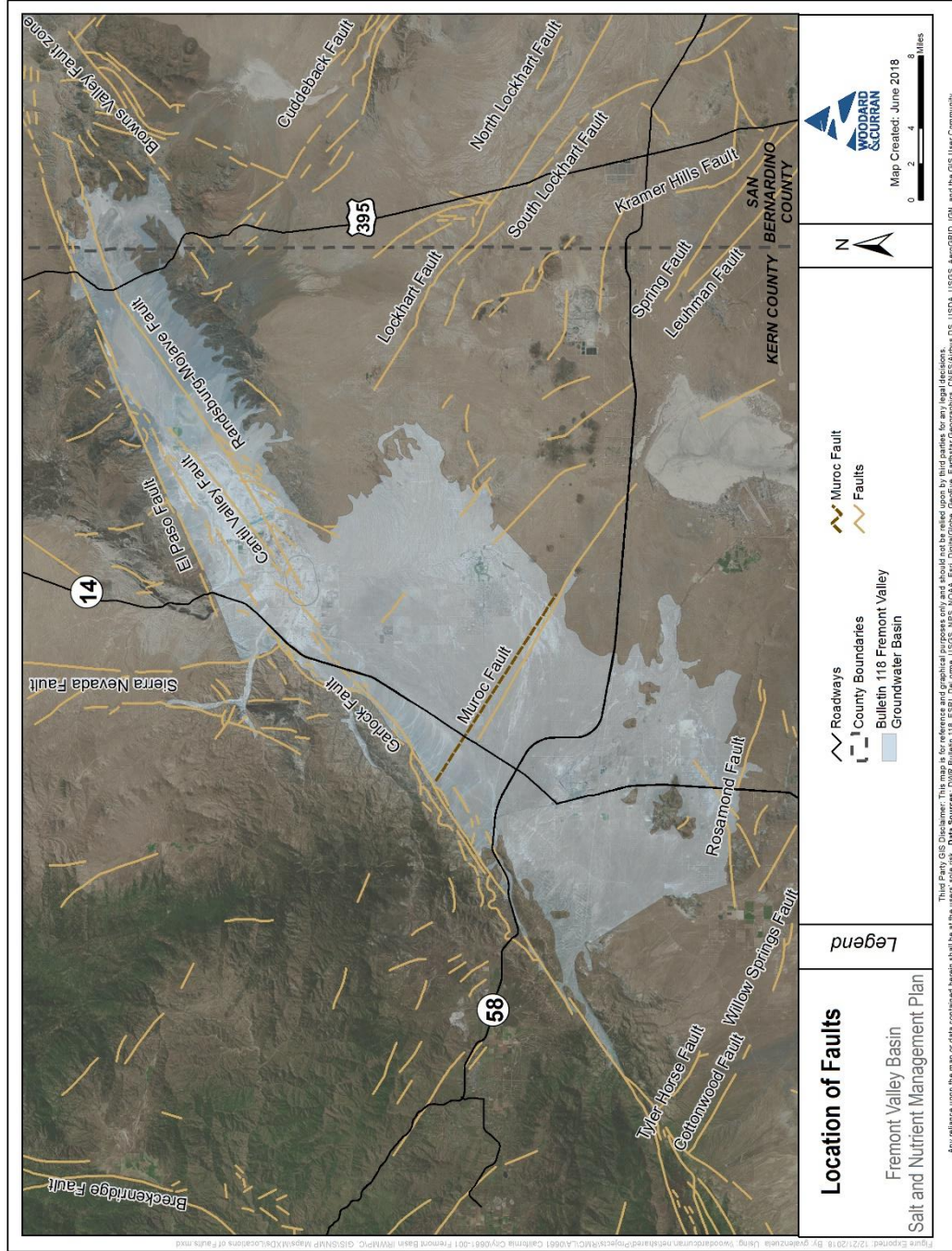
Figure 12: Location of Faults
