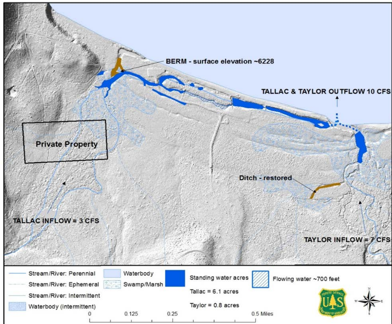
Figure 12. Restored wetland water area at base flow at low lake level (elevation 6224.0, U.S. Geological Survey water level datum).
