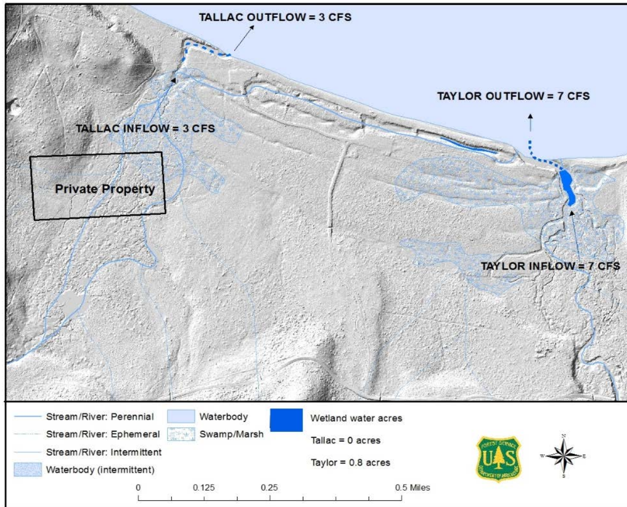
Figure 11. Existing wetland water area at base flow at low lake level (below elevation 6224.0 feet, U.S. Geological Survey water level datum).
