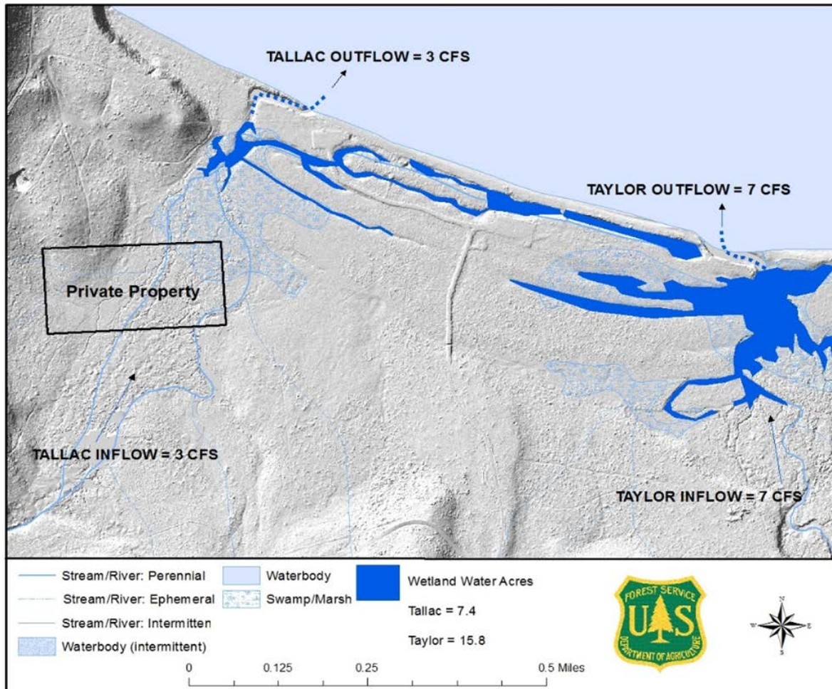
Figure 9. Existing wetland water area at base flow at median lake level (elevation 6226.8 feet, U.S. Geological Survey water level datum).
