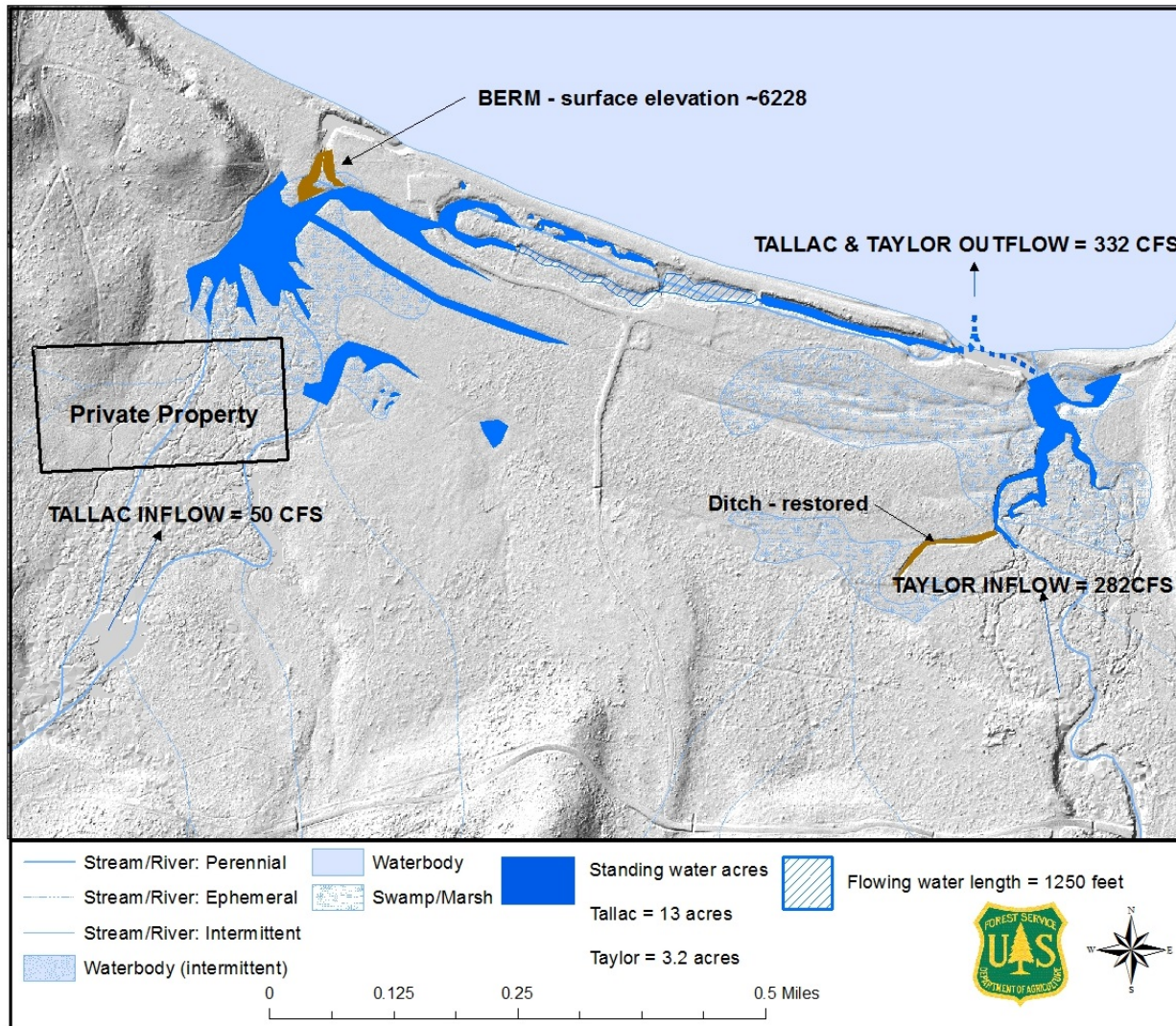
Figure 8. Restored wetland water area at bankfull flow at low lake level (below elevation 6224.0, U.S. Geological Survey water level datum).
