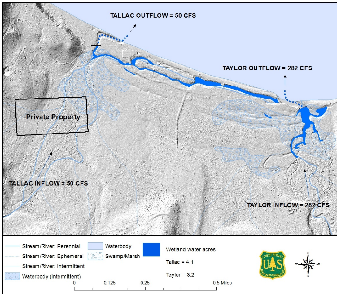
Figure 7. Existing wetland water area at bankfull flow at low lake level (below elevation 6224.0 feet, U.S. Geological Survey water level datum).
