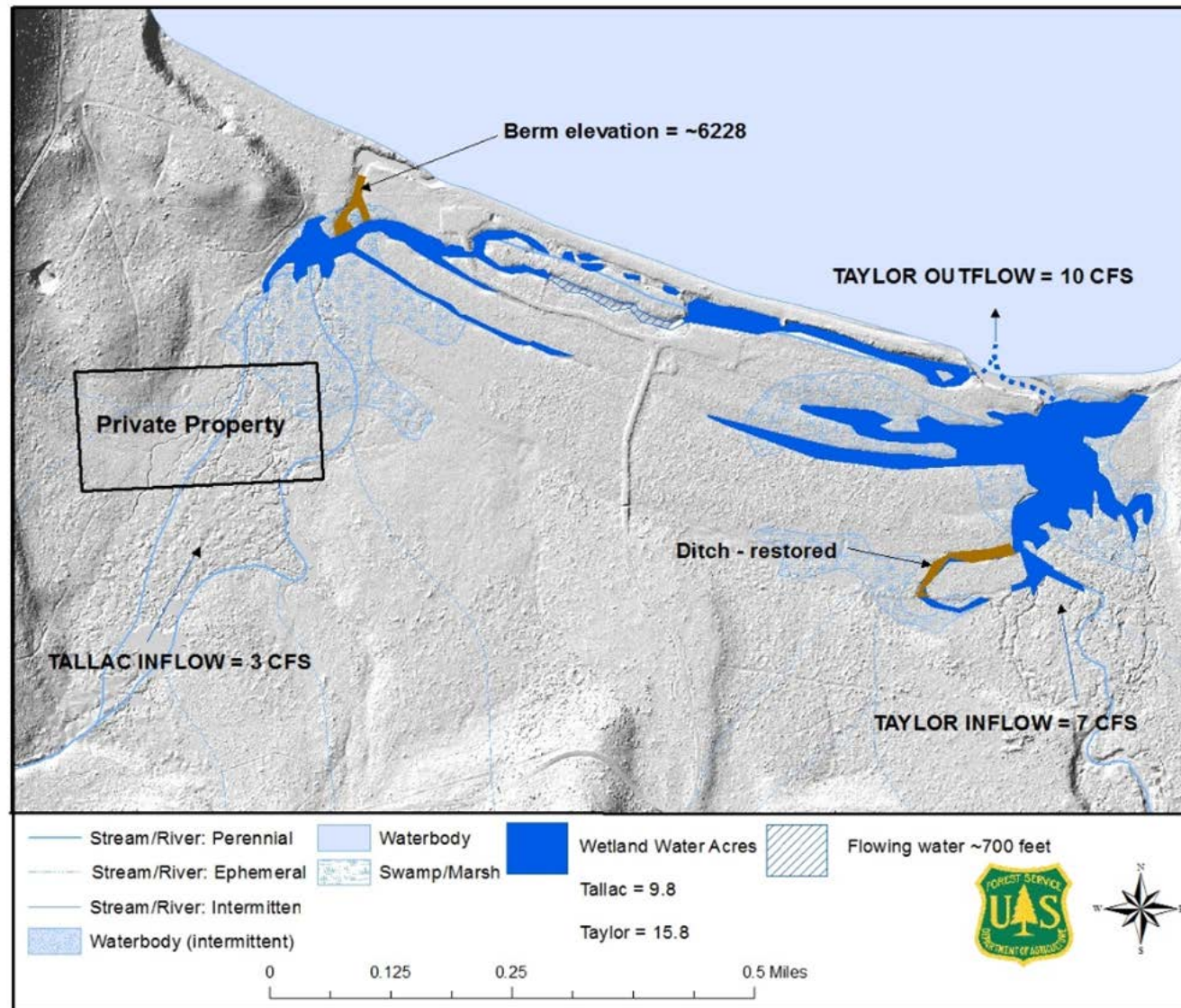
Figure 10. Restored wetland water area at base flow at median lake level (elevation 6226.8 feet, U.S. Geological Survey water level datum).
