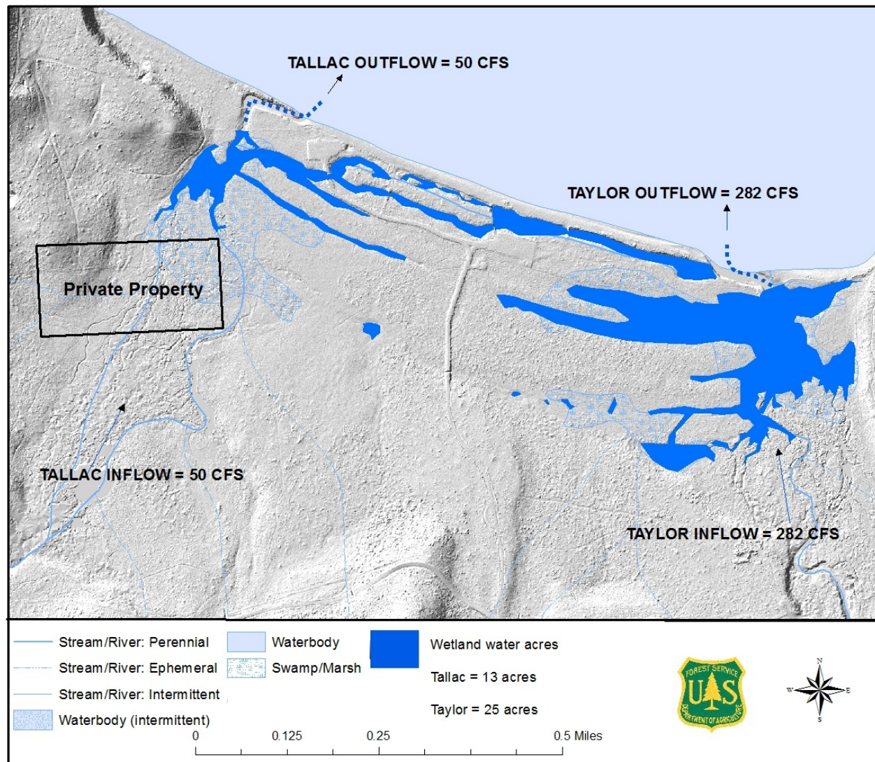
Figure 5. Existing wetland water area at bankfull flow at median lake level (elevation 6226.8 feet, U.S. Geological Survey water level datum).
