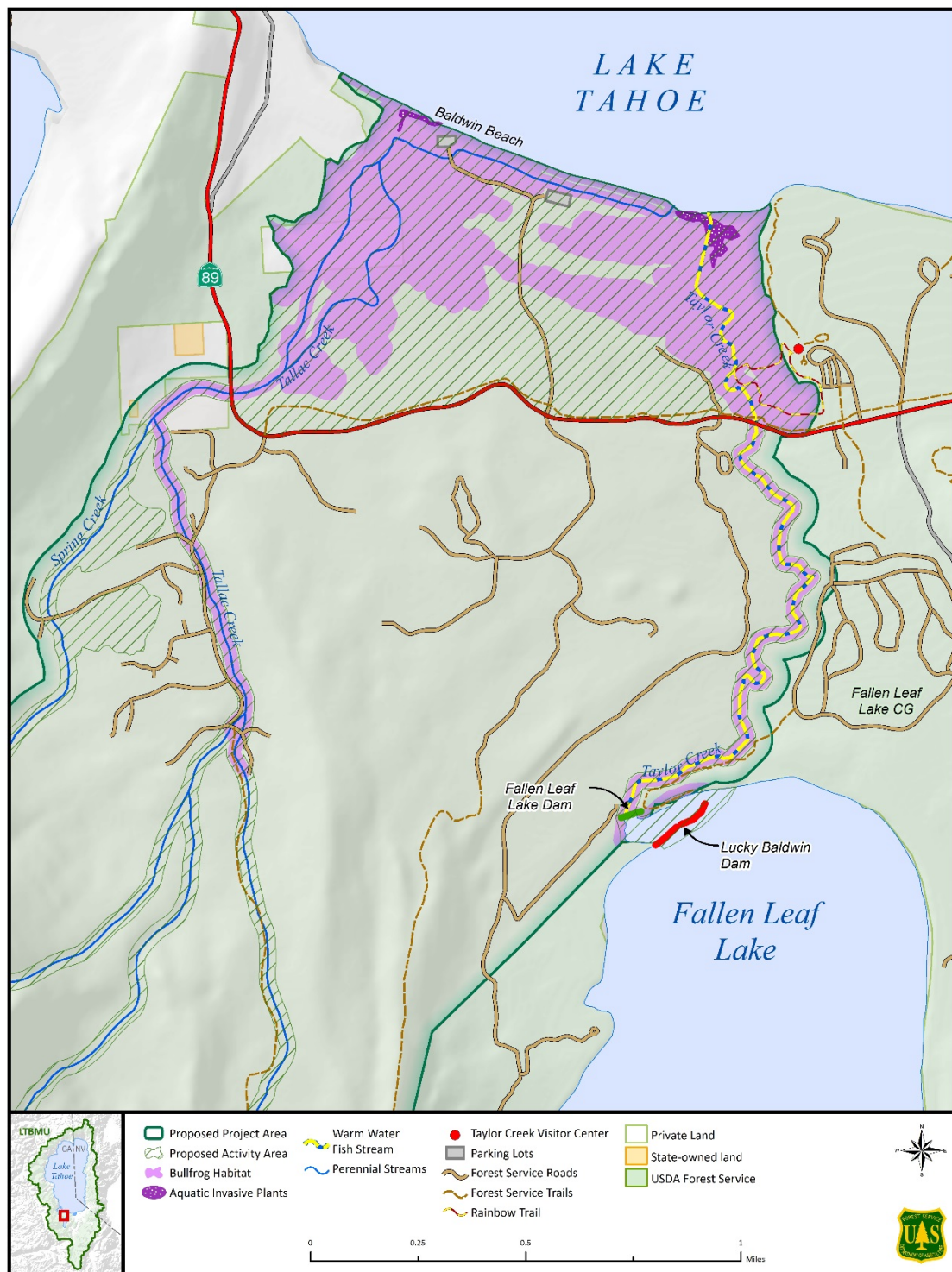
Figure 13. Current distribution of aquatic invasive species in the proposed project area.
