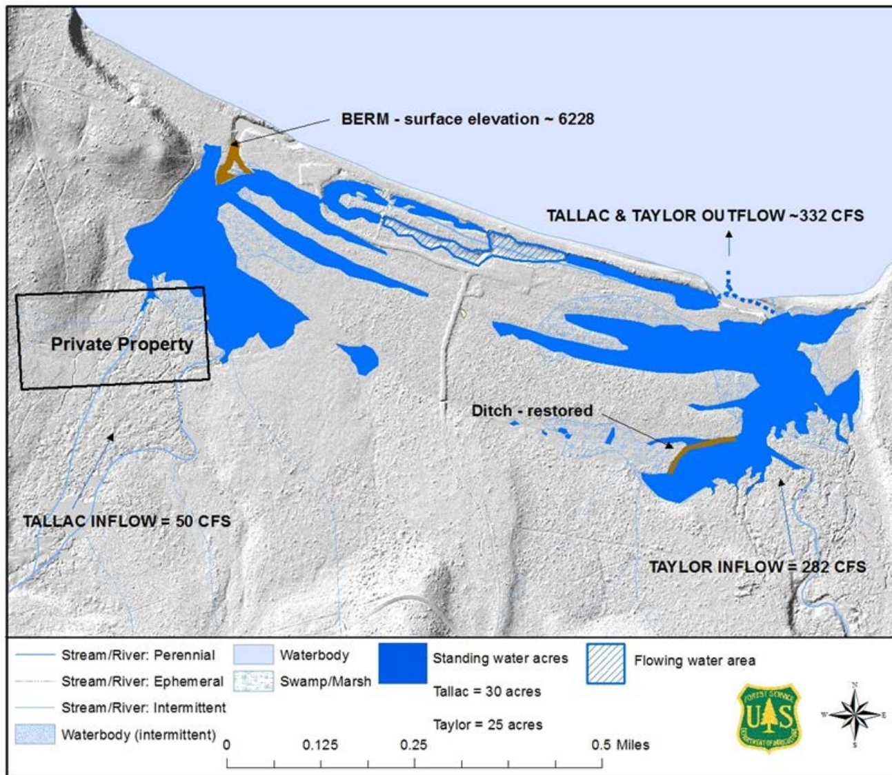
Figure 6. Restored wetland water area at bankfull flow at median lake level (elevation 6226.8 feet, U.S., Geological Survey water level datum).
