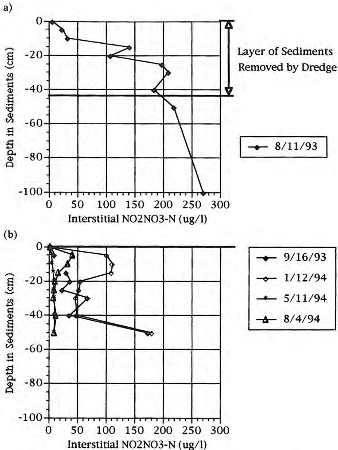
Figure 7-1. (a) Predredging profiles of sediment interstitial NO 2 NO 3 -N ( \mu\text{g/l} ) collected at Tahoe Keys core site #1 on 8/11/93; (b) postdredging profiles of sediment interstitial NO 2 NO 3 -N collected 9/16/93, 1/12/94, 5/11/94, 8/4/94.
