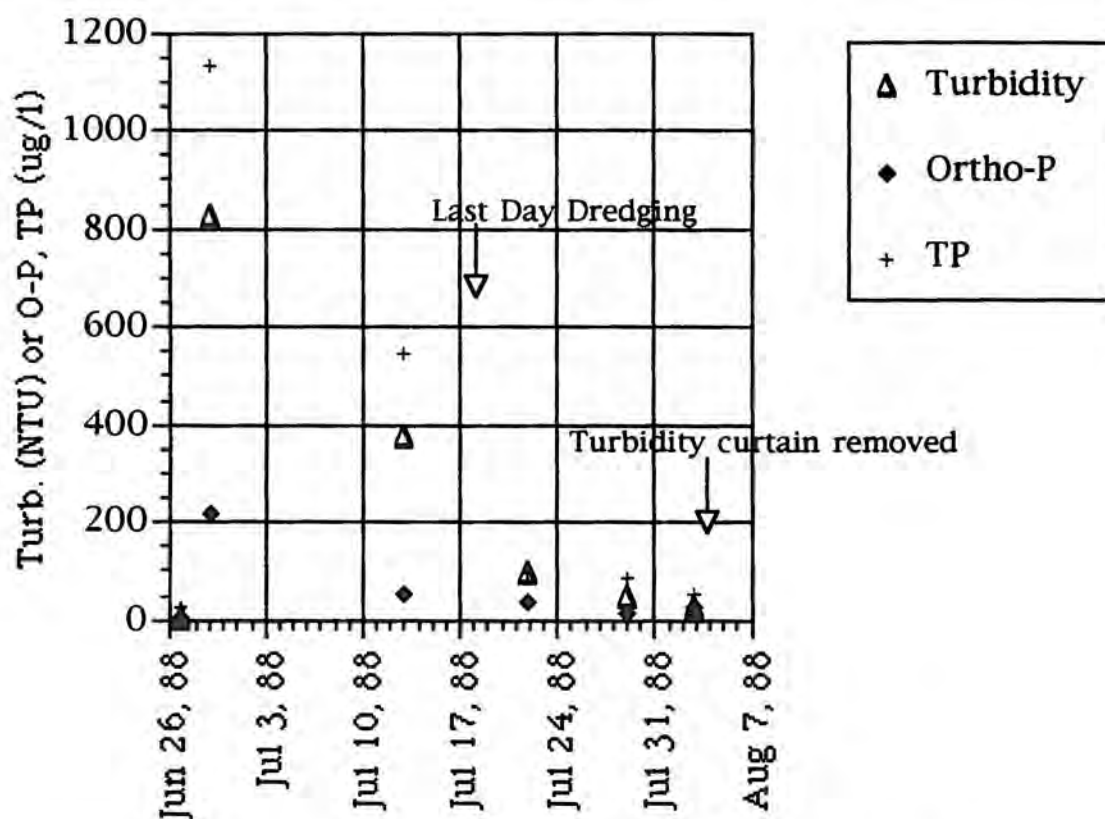
Figure C-3. Levels of turbidity, Ortho-P and TP within the silt curtain enclosed area during dredging at the Tahoe Boat Co. Marina, 1988.
