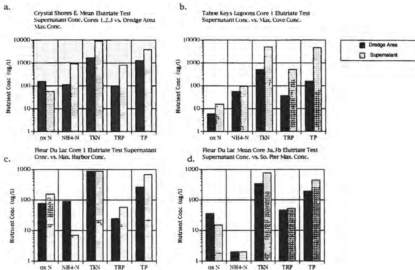
Figure 4-6. Plots of maximum concentrations of oxidized N, NH 4 -N, TKN, TRP, and TP observed in silt curtain enclosed dredging areas versus mean concentrations of these nutrients in elutriate test supernatant solution for cores collected within the following dredging areas: (a) Crystal Shores East; (b) a side cove in Tahoe Keys lagoons enclosed by silt curtain; (c) Fleur Du Lac harbor; (d) Fleur Du Lac south pier area.
