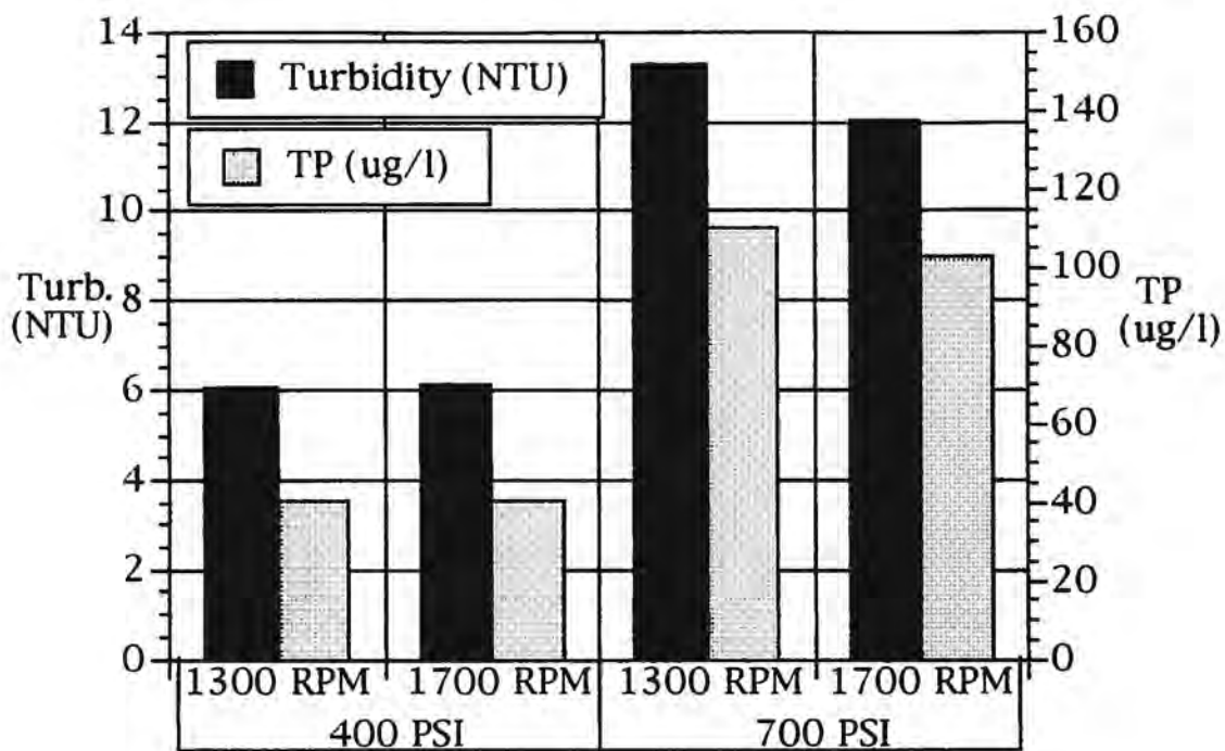
Figure 4-3. Mean turbidity and TP around the VMI 612 hydraulic dredge at different combinations of engine RPM and auger pressure (PSI) during testing in the Tahoe Keys Marina. Water samples were collected at locations 10 ft. ahead of the left and right sides of the cutterhead, and 10 ft. perpendicular to the cutterhead, at three depths: near the surface, mid-water column, and near the bottom. Means were calculated from all data collected for a combination engine RPM and auger pressure PSI. (Note: data for sample "D"-4 ft. collected at 1700 RPM and 700 RPM was excluded from the calculations because the Van Dorn bottle appeared to contact the bottom and collect some bottom sediments).
