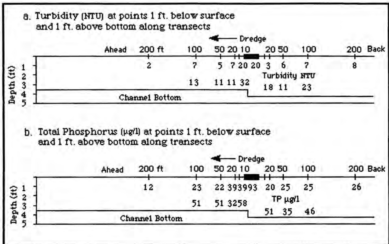
Figure 4-1. Turbidity and TP concentrations ahead of and behind the VMI 612 horizontal cutter hydraulic dredge. The dredge was operating in shallow open lake water, in the Tahoe Keys East Channel on 11/12/92
