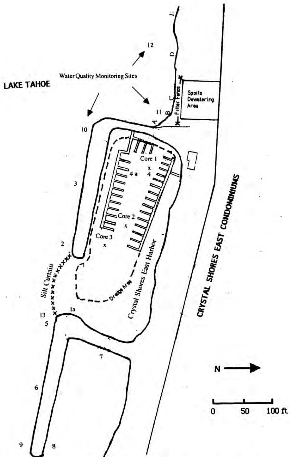
Appendix B-7. Locations of TRG water quality monitoring sites (#1-13), and shallow nearshore water collection sites (A-E) during excavator dredging at Crystal Shores East in 1993. Also shown are sediment coring locations.
