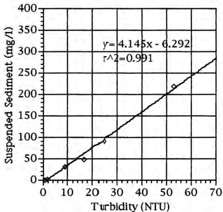
Figure D-1. Relationship between turbidity and suspended sediment for variable amounts of Tahoe Keys Marina sediments resuspended in lake water.
