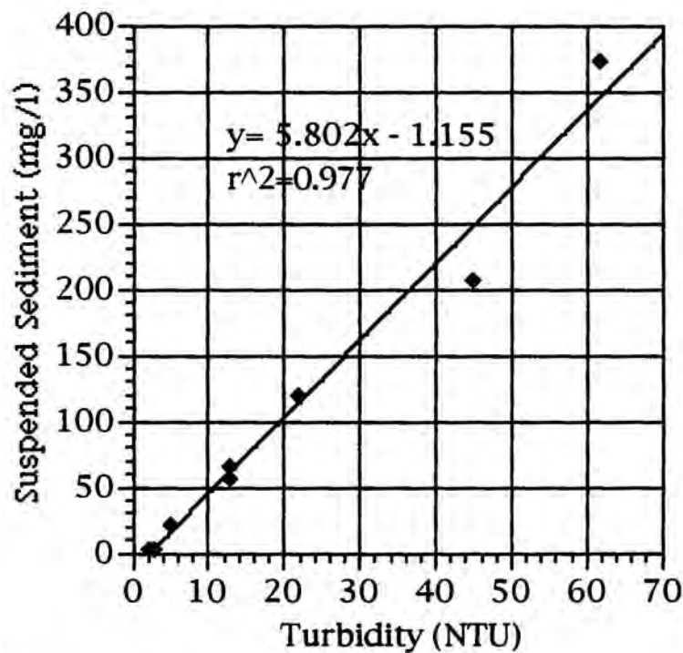
Figure D-2. Relationship between turbidity and suspended sediment for variable amounts of Crystal Shores East Harbor sediments resuspended in lake water.
