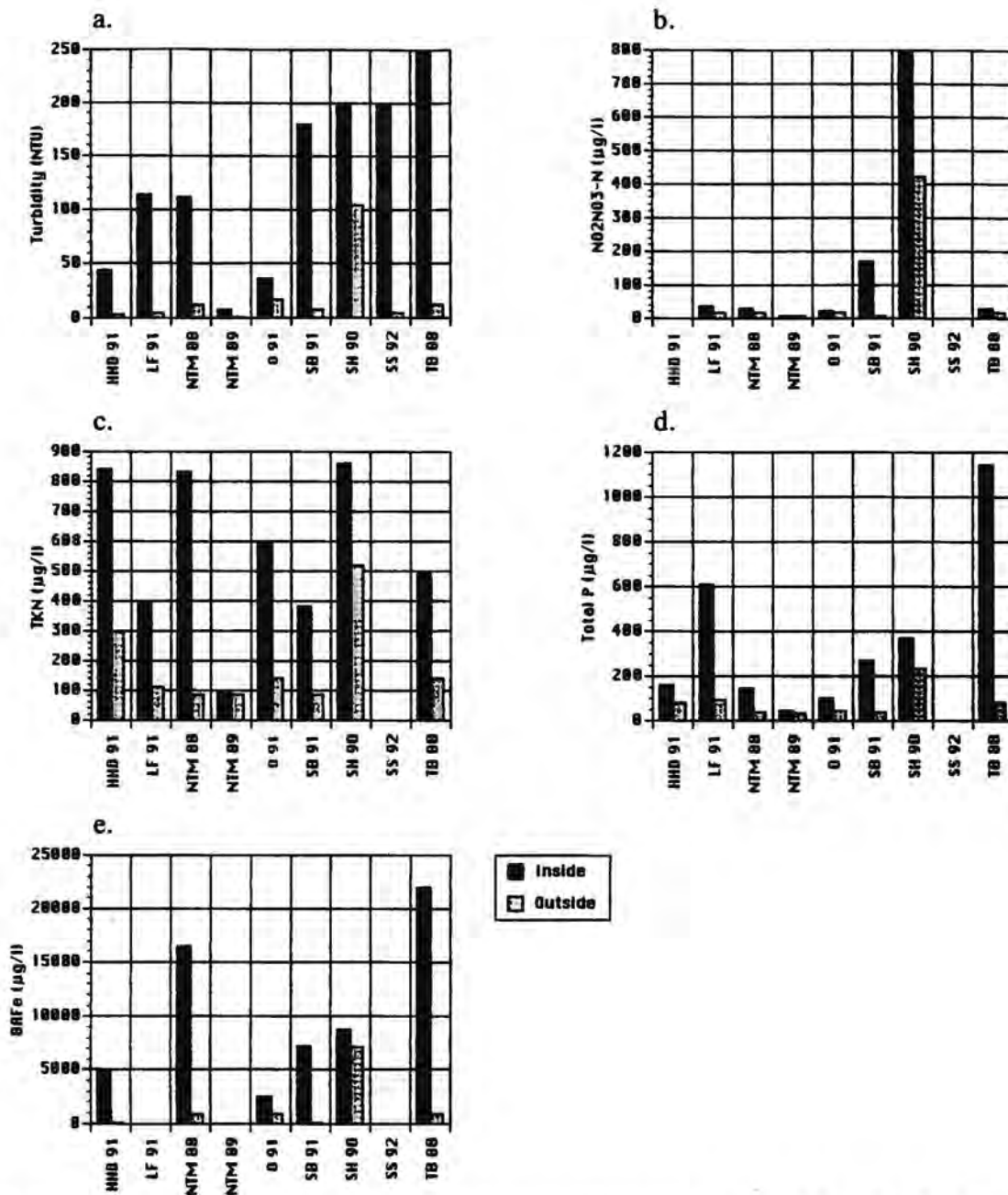
Figure C-4. Comparison of maximum observed levels of (a) turbidity, (b) NO 2 NO 3 -N, (c) TKN, (d) Total-P, (e) BAFe within and outside of silt curtain enclosed areas during historical dredging projects (HHD=Homewood High and Dry Marina, LF=Lake Forest Boat Ramp, NTM=North Tahoe Marina, O=Obexer's Marina, SB=Sierra Boat Co. Marina, SH=Star Harbor, SS=Sunnyside Marina, TB=Tahoe Boat Co. Marina).
