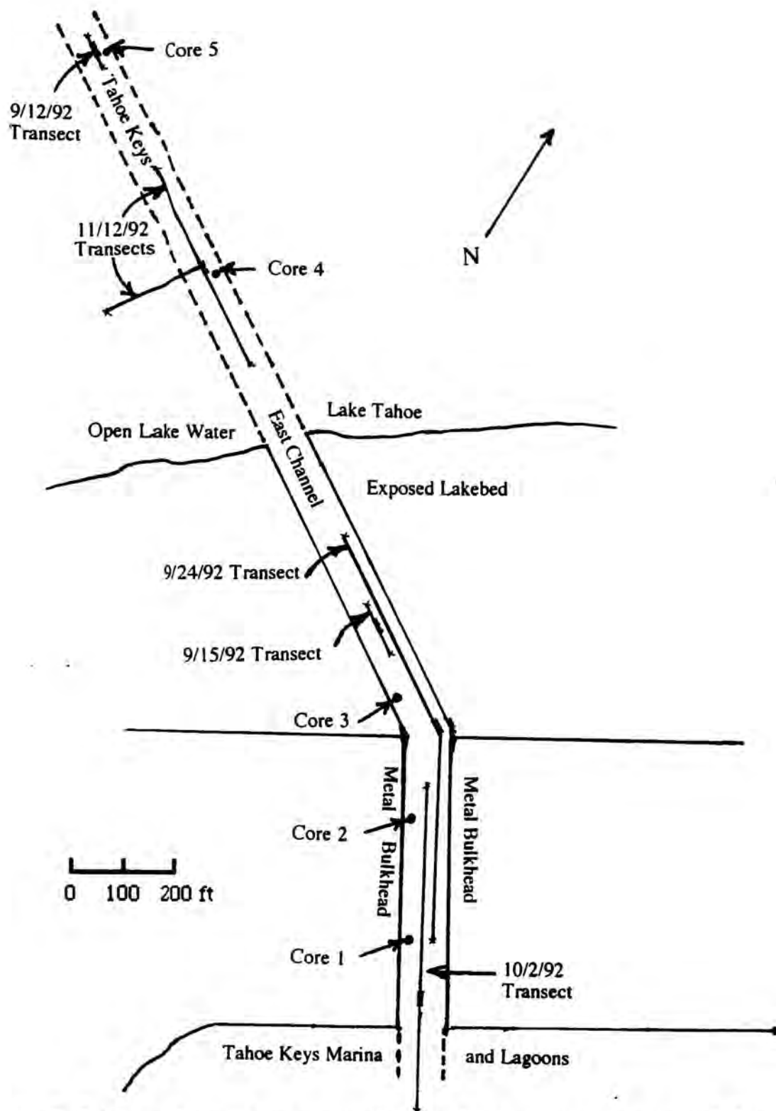
Appendix B-2. Locations of water quality monitoring transects around the VMI 612 horizontal cutter during operations in the Tahoe Keys East Channel in 1992. Also shown are locations of predredging sediment cores collected by Chemax Labs, Sparks, Nv. and the TRG on 7/8/92.
