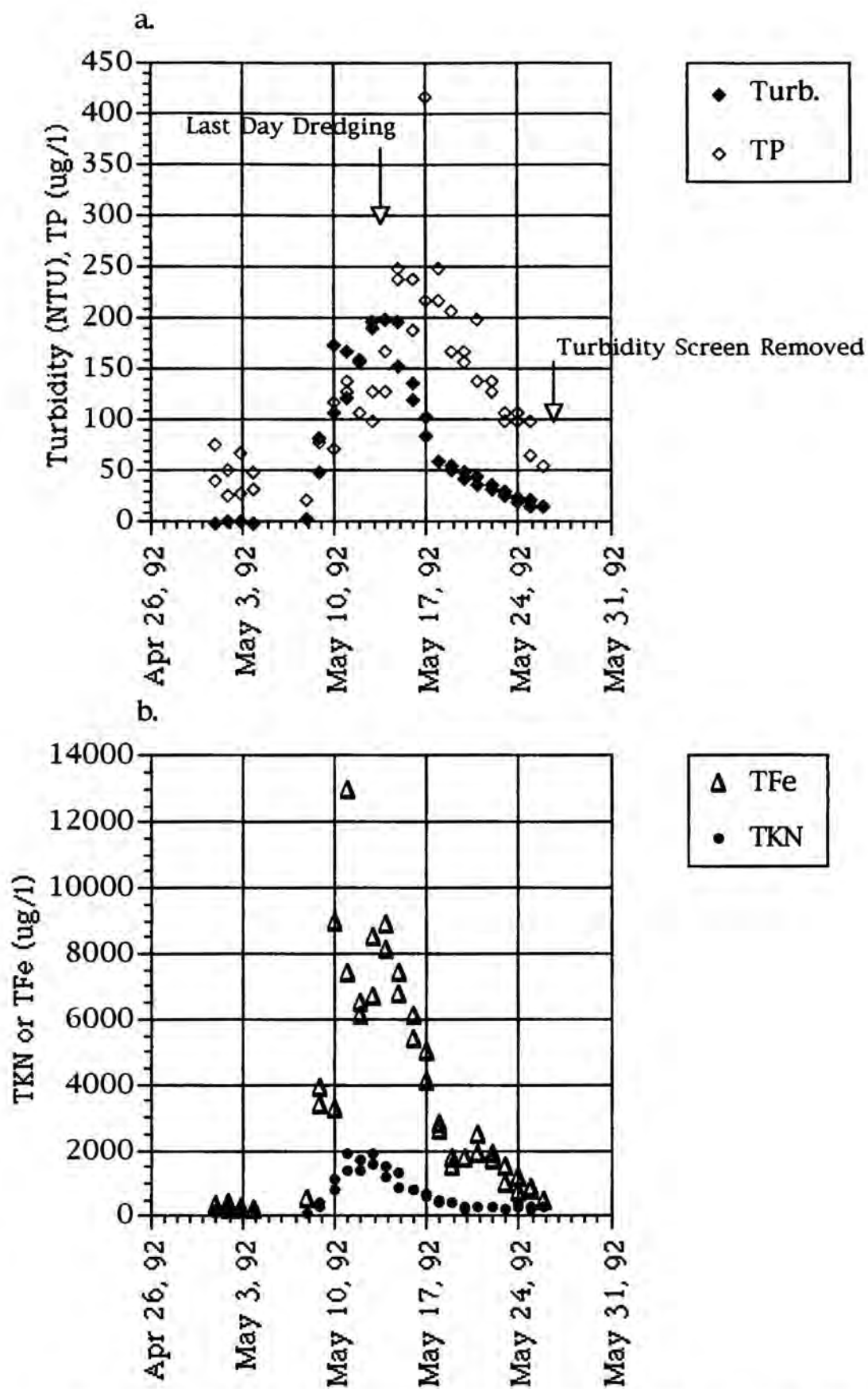
Figure C-1. Levels of (a) turbidity and TP; (b) TKN and TFe within the silt curtain enclosed harbor during dredging at Sunnyside Marina 1992.
