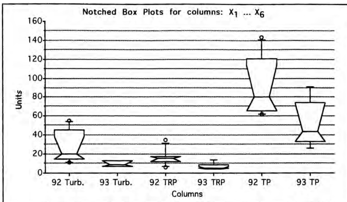
Figure 5-2 (a). Notched box plot comparison of 1992 versus 1993 levels of turbidity, TRP, and TP in Tahoe Keys impoundment basin (Pond) 3, Site 7. Units for turbidity are NTU and units for nutrients are \mu\text{g/l} . In 1992, spoils from the dredge were discharged directly into the impoundment basins. In 1993, sands and larger particulates were removed from the spoils first using a sand classification system, then alum was added to the remaining stream of dredge slurry as it was discharged to the impoundment basins. Box plots are interpreted as follows: the median value for each parameter is indicated by the middle line in each "box"; the notches in the "box" represent the 95% confidence intervals of the median; the top of the "box" represents the 75th percentile value; the bottom of the "box" represents the 25th percentile; the "tic" mark connected to the top of the box by a line represents the 90th percentile value; similarly the "tic" mark connected to the bottom of the box by a line represents the 10th percentile value; outlying points are indicated as circles. Data from 9/4/92, 9/10/92, 9/11/92 was excluded from these calculations since the ponds had not yet stabilized (Pond 3 had unusually high turbidity and nutrient levels resulting from erosion of sediments from the weir); data from 8/25/93 was also excluded as a malfunction occurred with the alum + flocculent injection system which resulted in unusually high turbidity and nutrients in Pond 3 and prevented discharge on this date.
