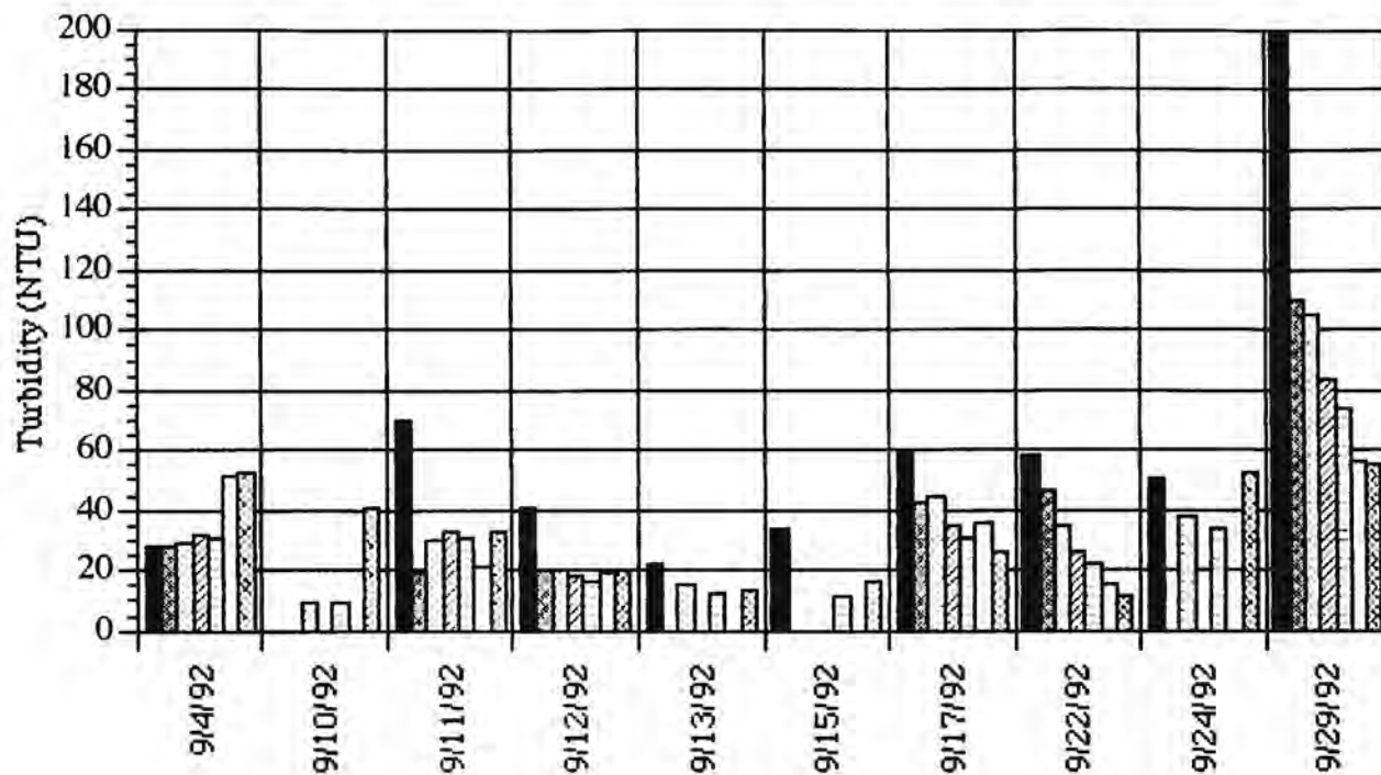
Figure 5-1 (c). Levels of turbidity at TRG monitoring sites within the Tahoe Keys spoils impoundment basins during hydraulic dredging in 1992.
