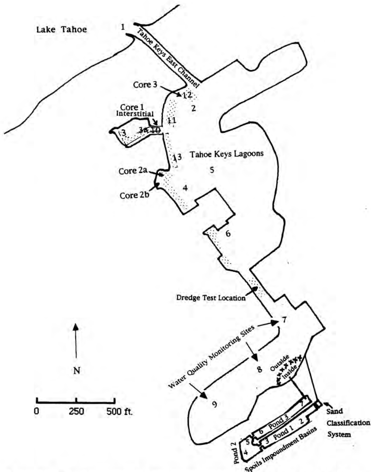
Appendix B-4. Locations of TRG water quality monitoring sites (#1-13), sediment coring locations, interstitial water collection site, and spoils impoundment basin monitoring sites during 1993 hydraulic dredging project in the Tahoe Keys Marina and lagoons. Also shown is the "Dredge Test Location" where sediment and nutrient resuspension produced by the VMI 612 dredge at varied operational control settings was monitored.
