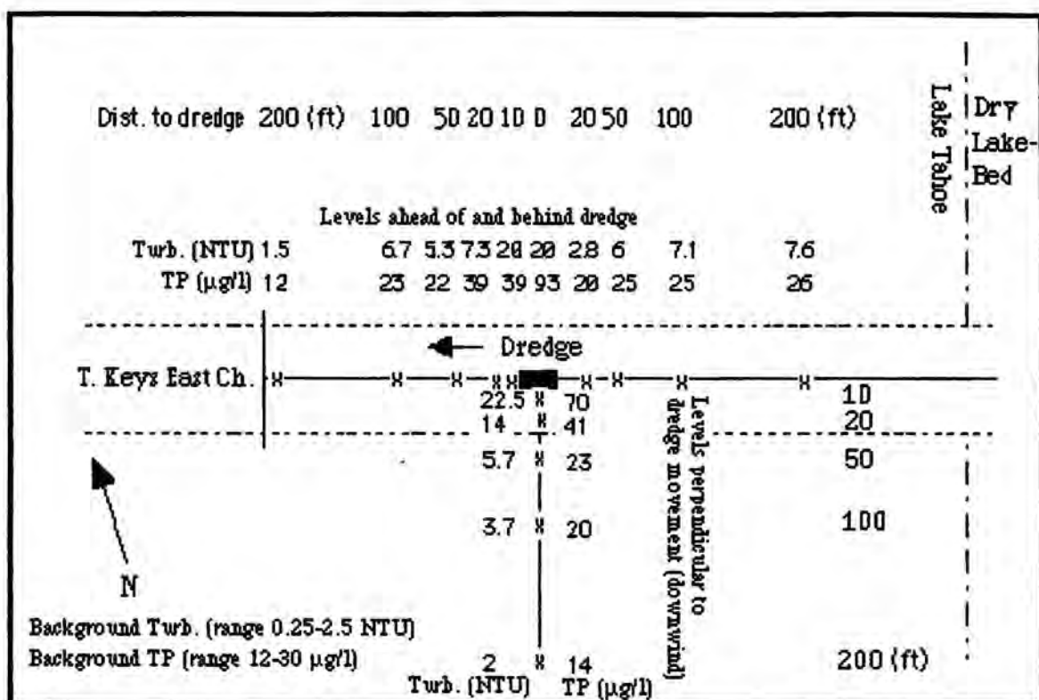
Figure 4-2. Near surface turbidity (NTU) and TP ( \mu\text{g/l} ) at sampling points "x" along transects ahead of, behind, and downwind of the VMI 612 hydraulic dredge. Samples were collected 11/12/92 in a shallow, open-lake section of the Tahoe Keys East Channel.
