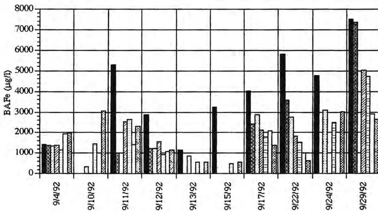
Figure 5-1 (f). Levels of BAFe at TRG monitoring sites within the Tahoe Keys spoils impoundment basins during hydraulic dredging in 1992.
