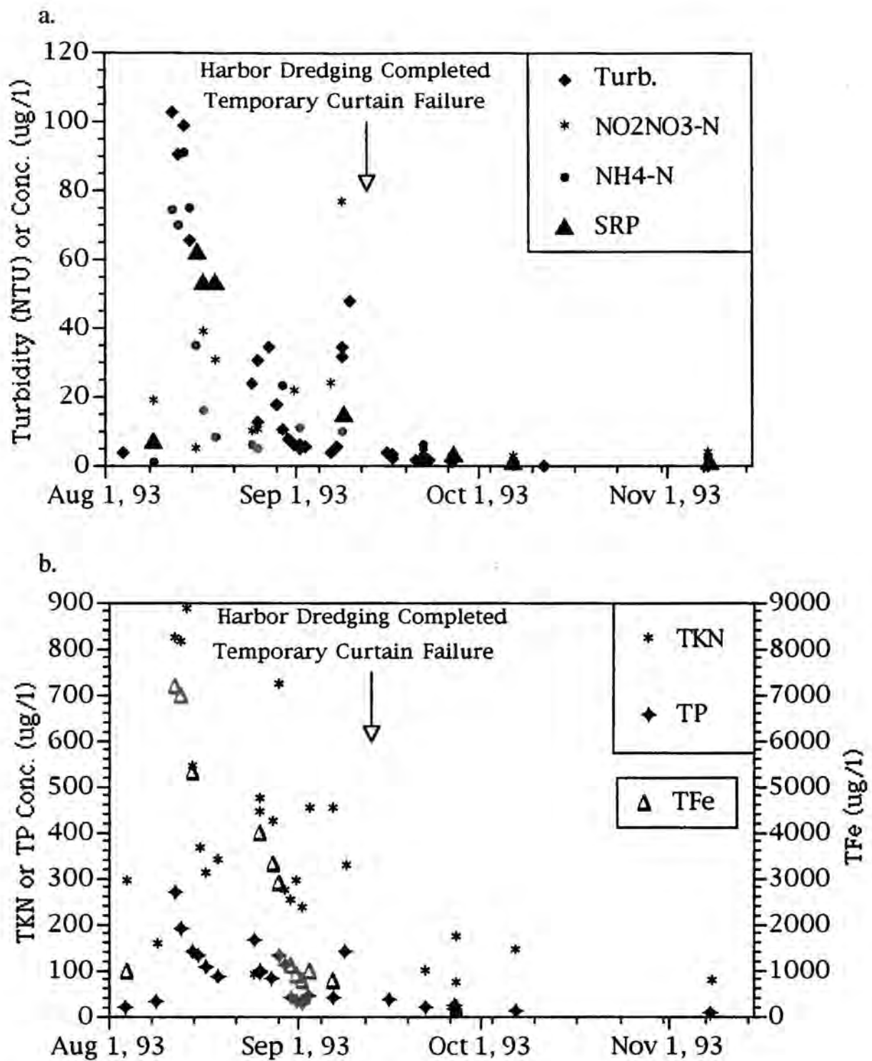
Figures 4-4 a, b. Patterns of turbidity and nutrient concentrations in the Fleur Du Lac harbor during and following the completion of dragline and clamshell dredging.
