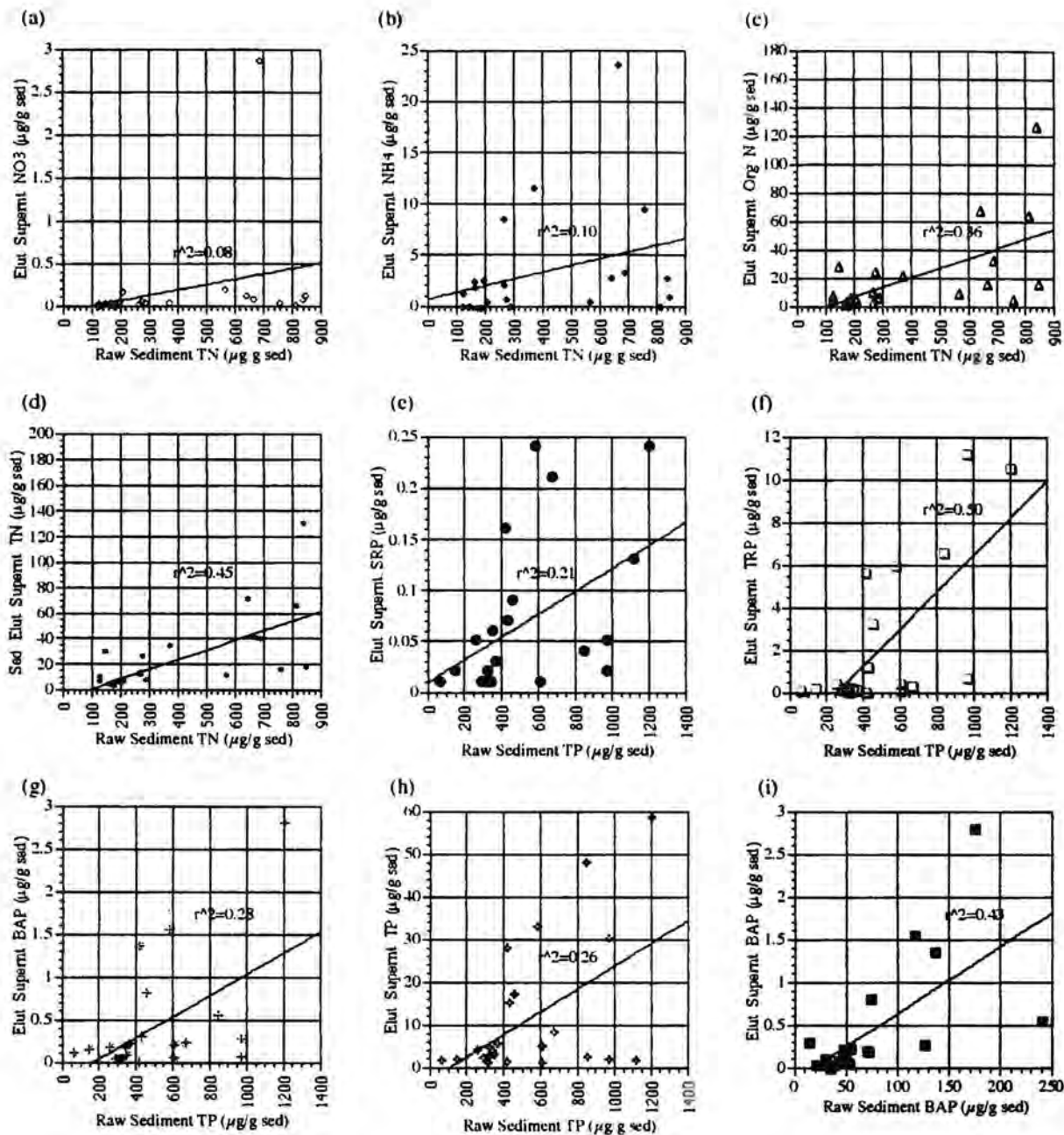
Figure 4-5. Associations between nutrients in dried core sediments and nutrients released into the supernatant solution in elutriate tests: (a) raw sediment TN vs. supernatant \text{NO}_3 ; (b) raw sediment TN vs. supernatant \text{NH}_4 ; (c) raw sediment TN vs. supernatant organic N; (d) raw sediment TN vs. supernatant TN; (e) raw sediment TP vs. supernatant SRP; (f) raw sediment TP vs. supernatant TRP; (g) raw sediment TP vs. supernatant BAP; (h) raw sediment TP vs. supernatant TP; (i) raw sediment BAP vs. supernatant BAP.
