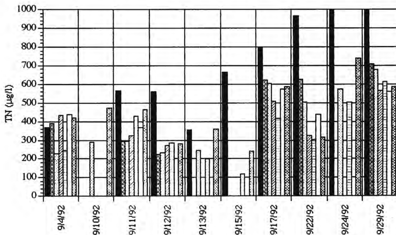
Figure 5-1 (d). Levels of TN at TRG monitoring sites within the Tahoe Keys spoils impoundment basins during hydraulic dredging in 1992.
