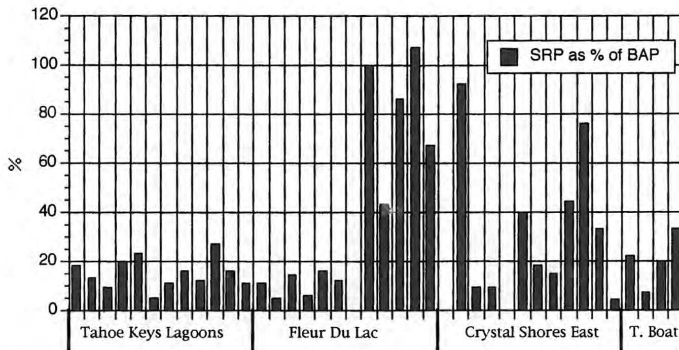
Figure 3-2. Comparison of SRP vs. BAP in sediment elutriate supernatant solutions from core sections from project sites. SRP is shown as percent of BAP concentration.
