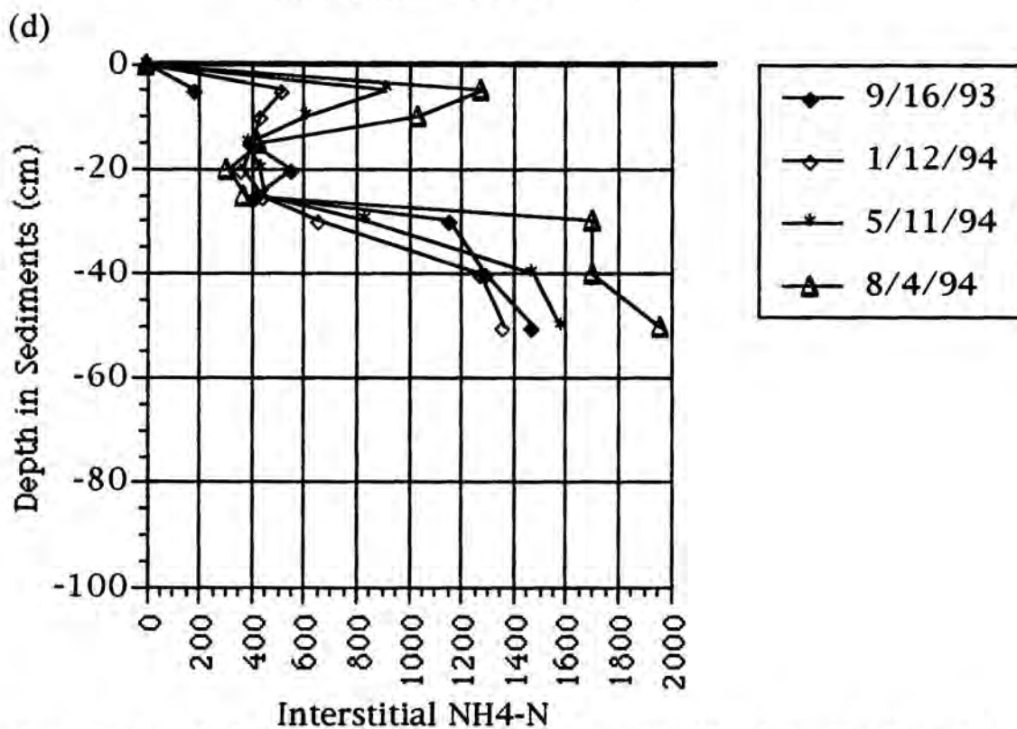
Figure 7-1. (c) Predredging profiles of sediment interstitial NH 4 -N (μg/l) collected at Tahoe Keys core site #1 on 8/11/93; (d) postdredging profiles of sediment interstitial NH 4 -N (μg/l) collected 9/16/93, 1/12/94, 5/11/94, 8/4/94.
