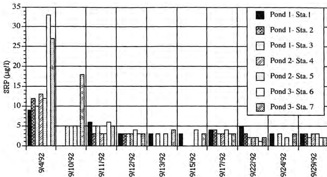
Figure 5-1 (a). Levels of SRP at TRG monitoring sites within the Tahoe Keys spoils impoundment basins during hydraulic dredging in 1992.
