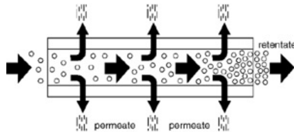
Figure 3-9. Crossflow microfiltration membrane tube diagram.
