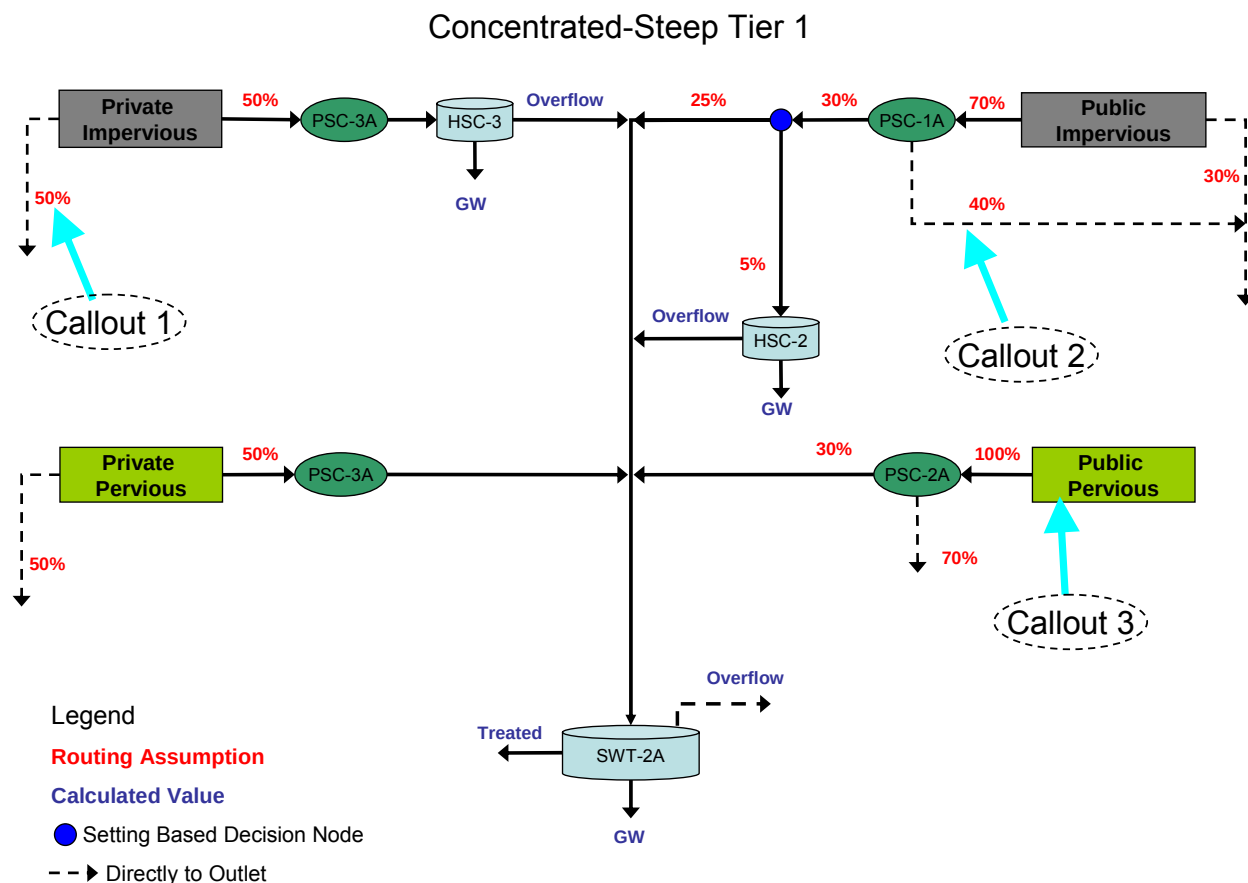
Figure 3-13. Analysis methodology to inform Input Tables for Tier 1.
