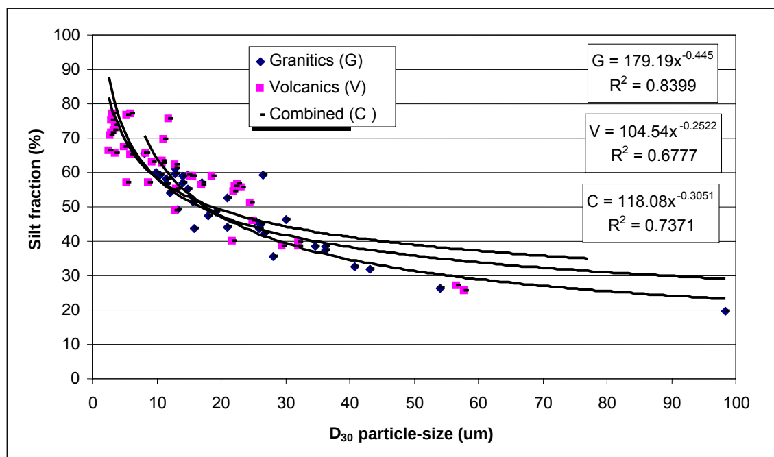
Figure 4-5. Dependence of silt fraction on D_{30} particle size for runoff from all soils.
