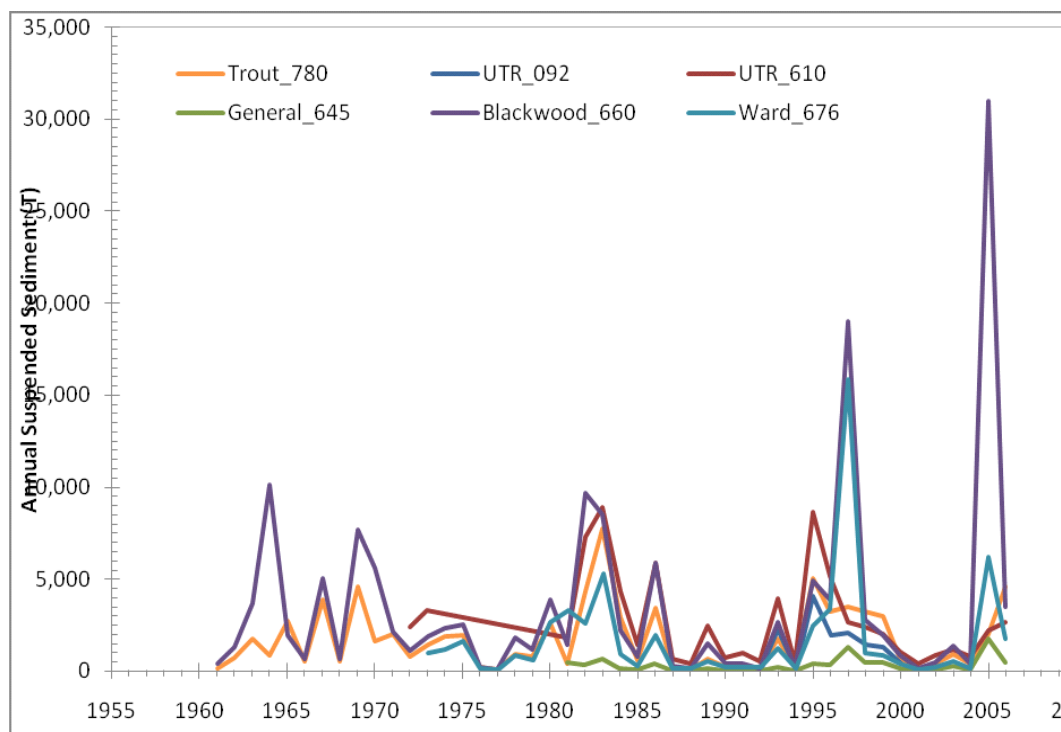
Figure 5-4. Annual suspended sediment (TSS) loads (MT) for major fine sediment source Tahoe streams
