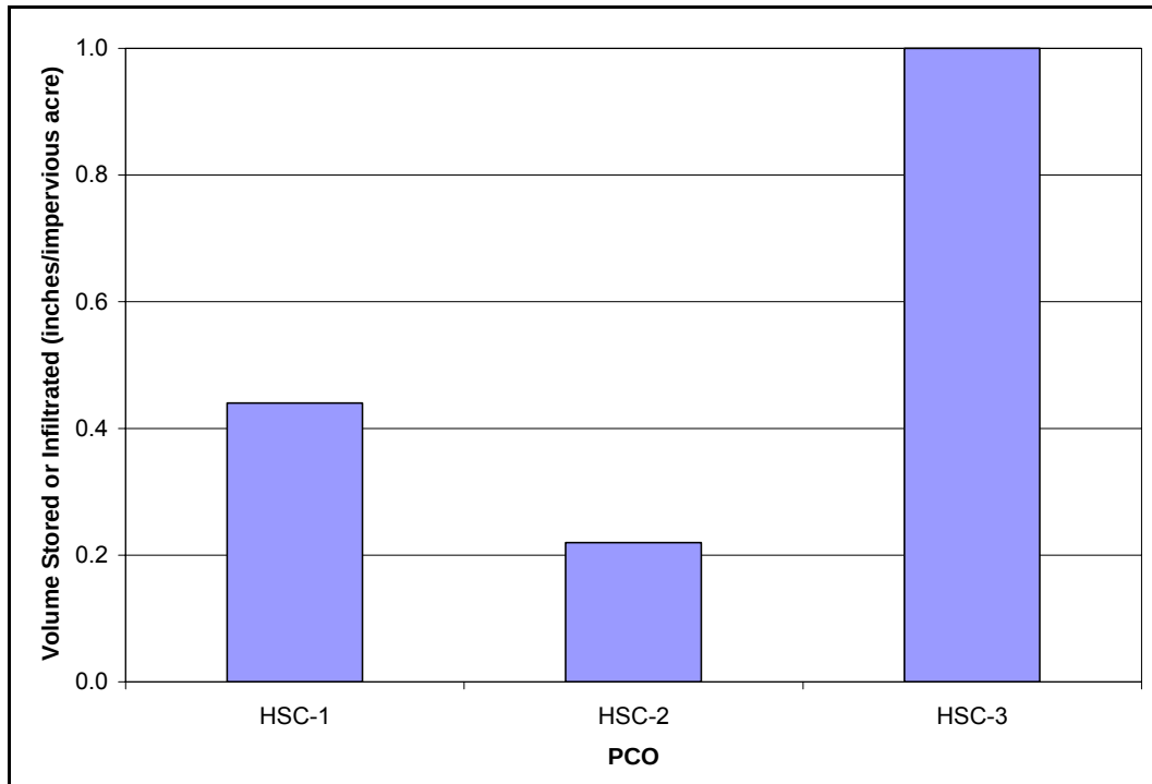
Figure 3-2. Volume of runoff stored or infiltrated in a 1-hour time step.
