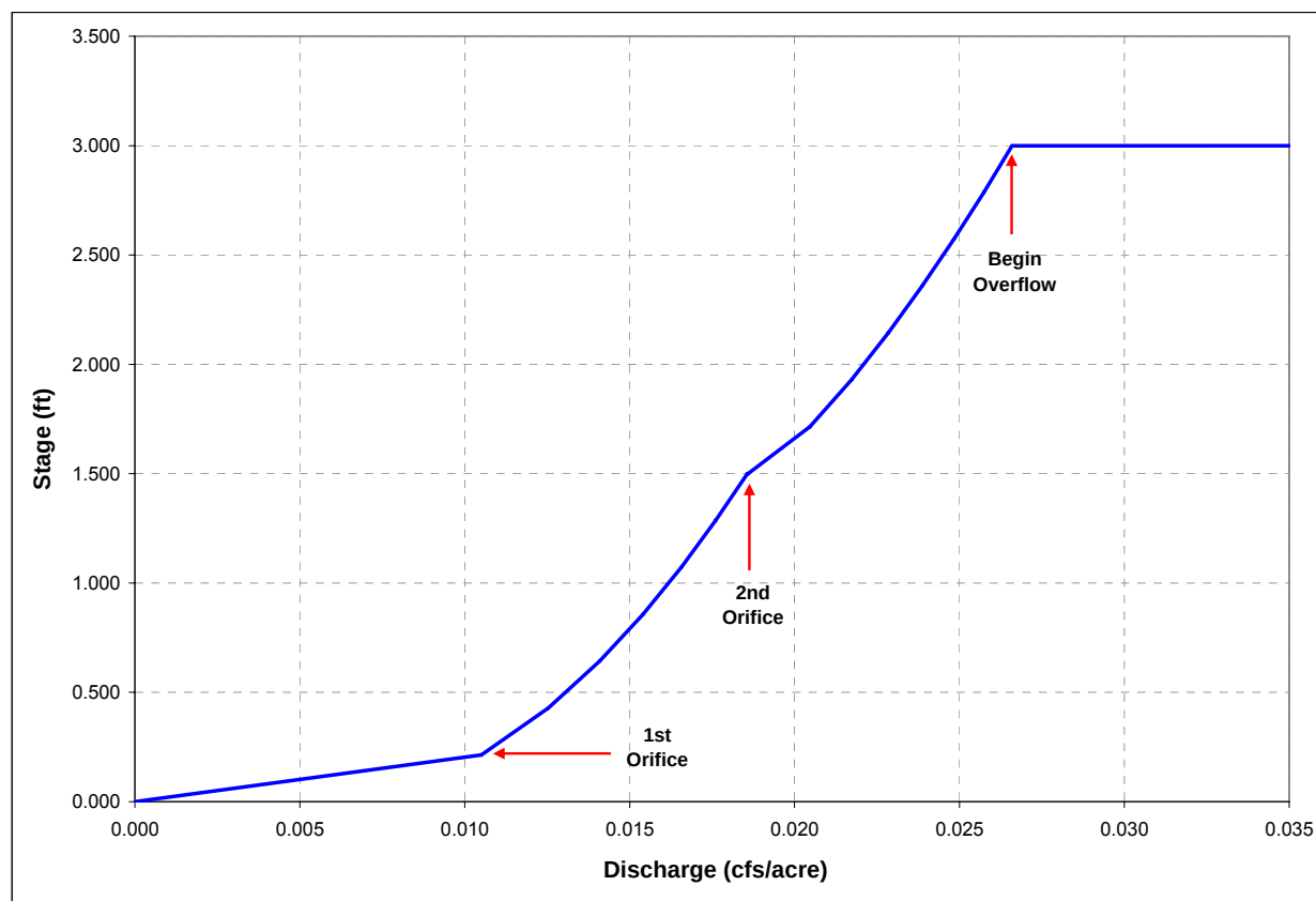
Figure 3-14. Stage-discharge relationship for two-stage drain time.
