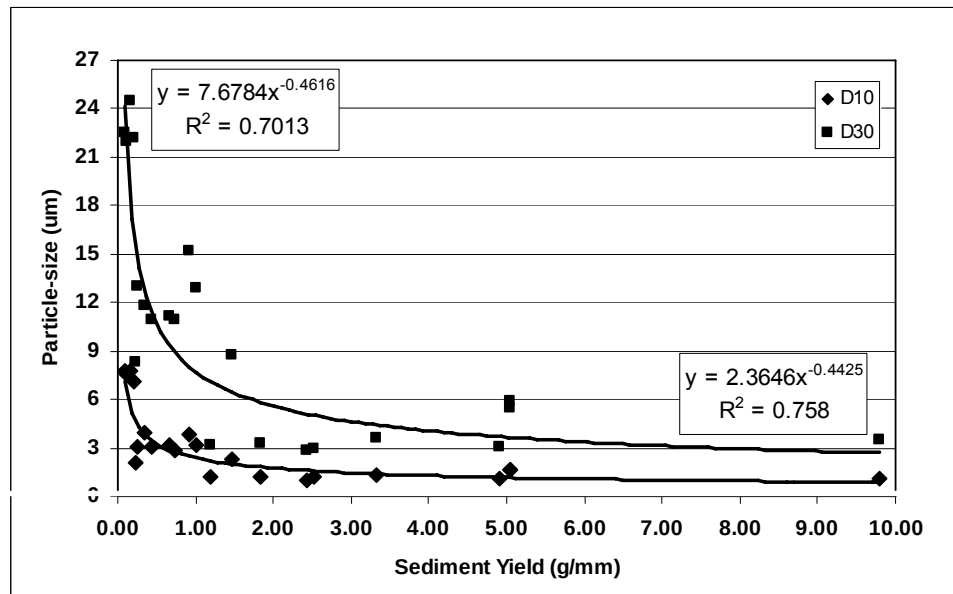
Figure 4-4. Dependence of silt and clay fractions on SY for runoff from volcanic soils.
