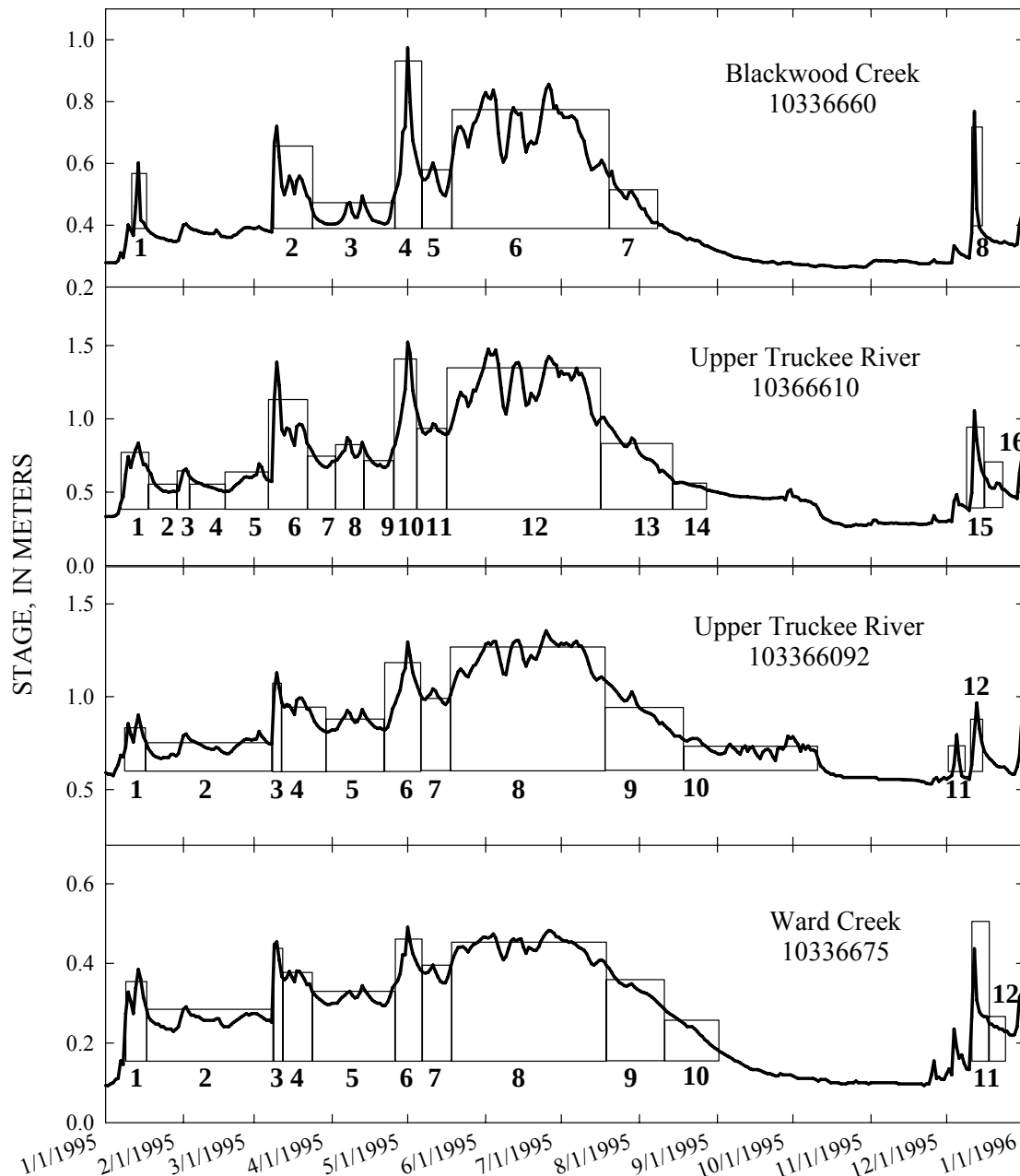
Figure 5-5. Simplified 1995 hydrographs for the four USGS gauging stations with numbered events used as input to the toe-erosion sub-model of BSTEM.
