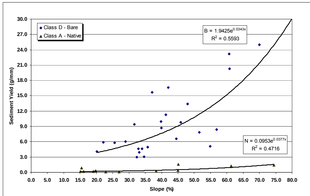
Figure 4-3. Example sediment yield (SY) versus slope regression equations for two treatment levels/functional classes on volcanic soils.
