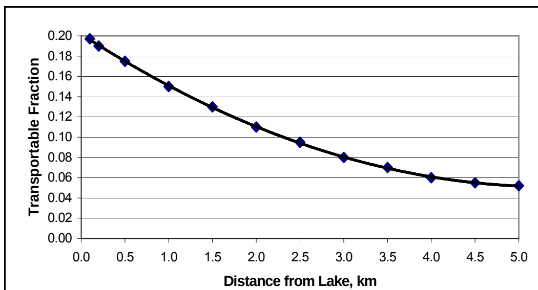
Figure 2-5. Transport fraction of fugitive dust versus distance from Lake
