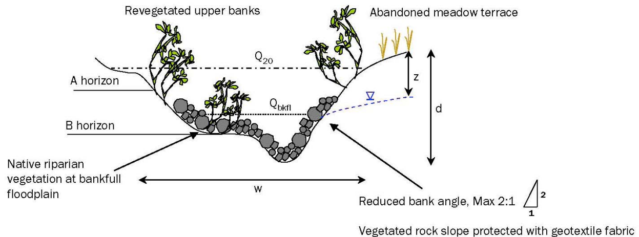
Figure 5-3. Schematic representation of Tahoe Basin stream channel characteristics under the Tier 3-bank protection conditions
