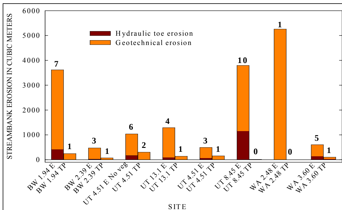
Figure 5-6. Simulated volumes of streambank erosion by hydraulic (toe erosion) and geotechnical (bank failure) processes.
