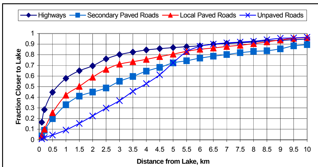
Figure 2-2. Cumulative distribution of VMT for paved and unpaved roads in the Basin
