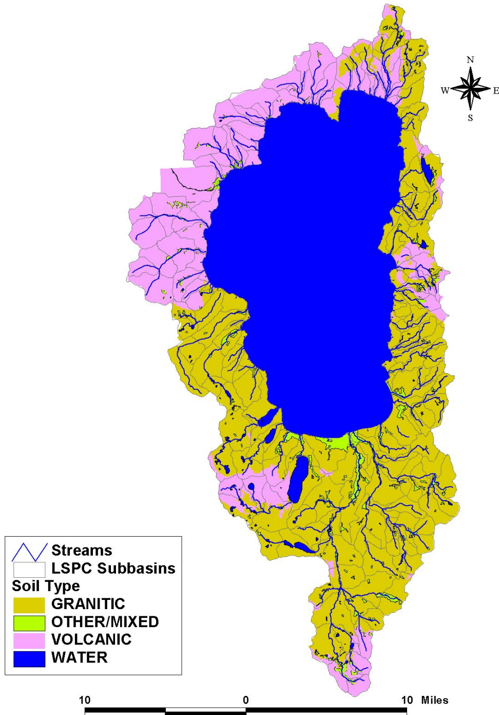
Figure 4-1. Soil parent material types in the Lake Tahoe Basin.
