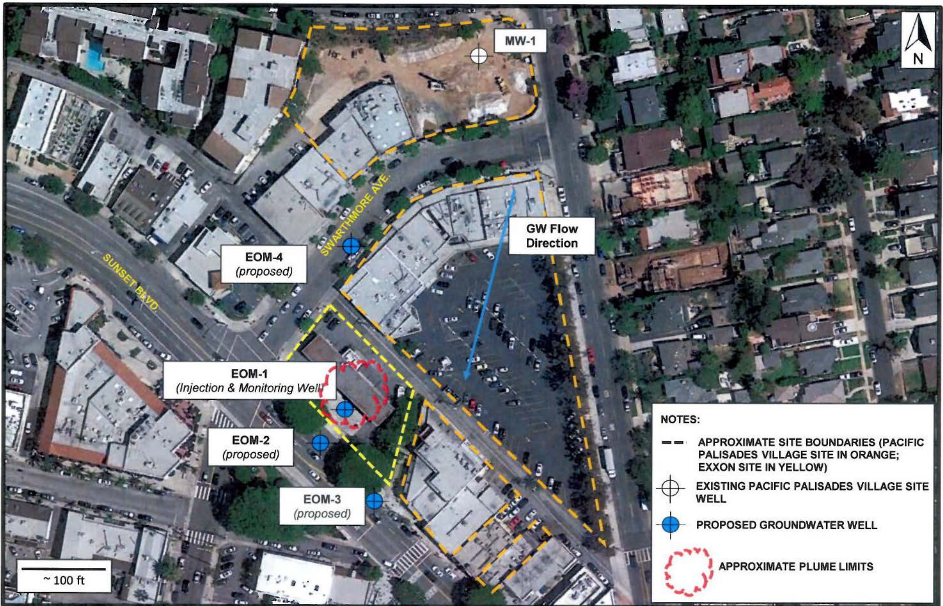
FIGURE 2 PROPOSED GROUNDWATER MONITORING WELL NETWORK
