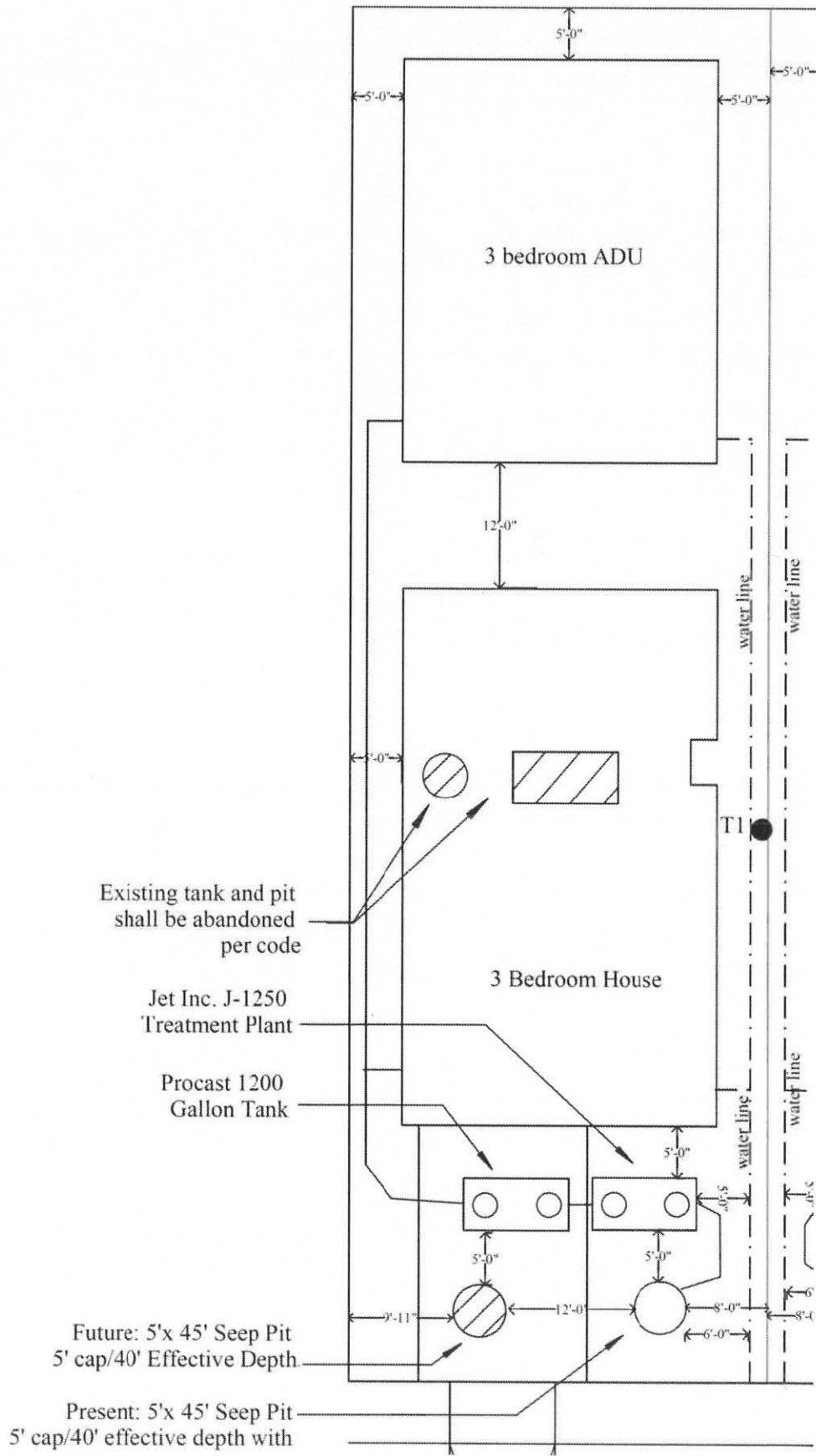
FIGURE 1 – OWTS Site Plan
