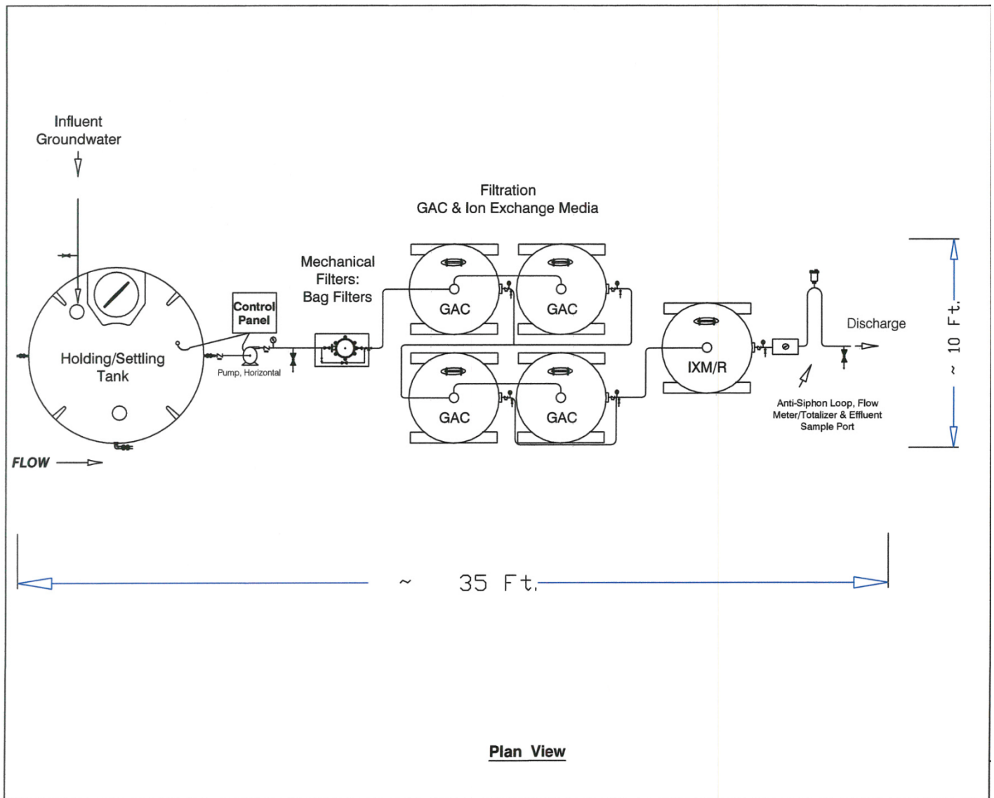
Figure 2. Treatment Process
