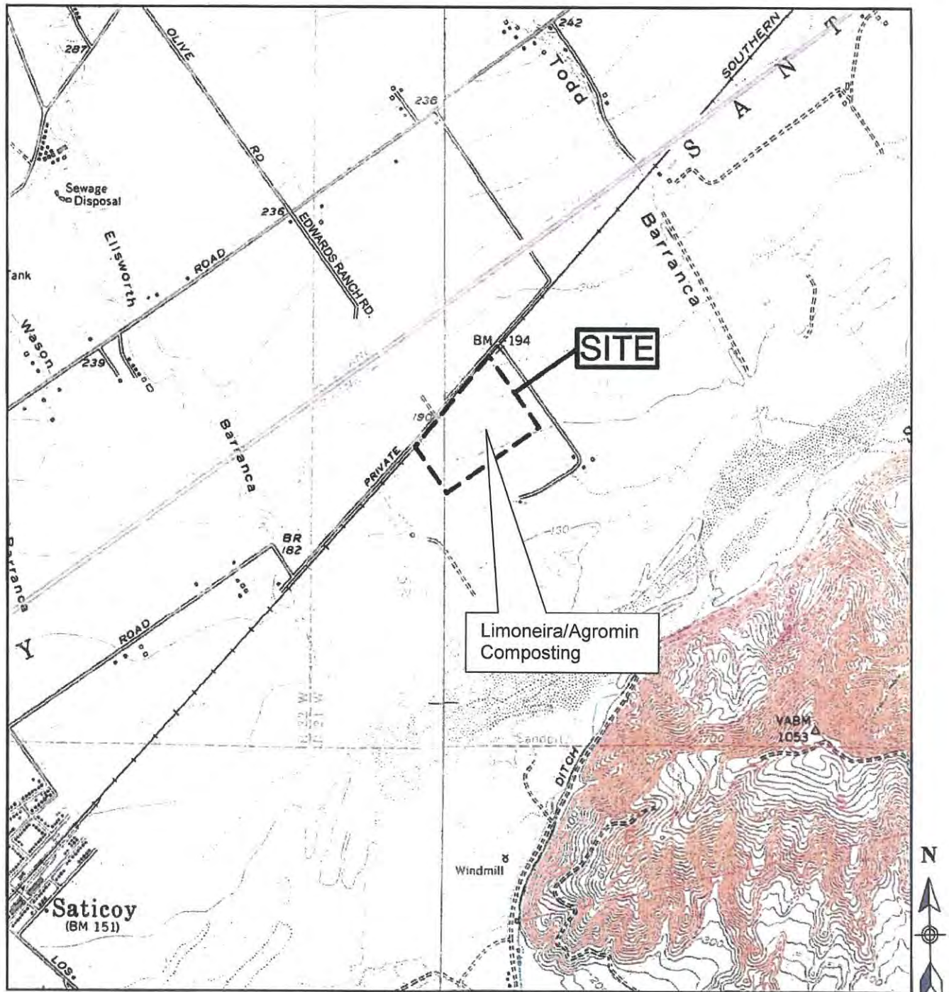
Base Map: USGS 7.5' Topographic Maps of the Saticoy and Santa Paula Quadrangles, 1967 Scale: 1 in. = 2,000 ft.
