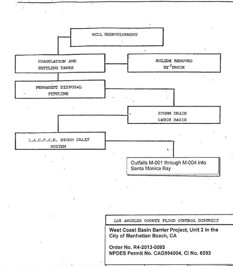
Figure 2. Schematic of Water Flow
