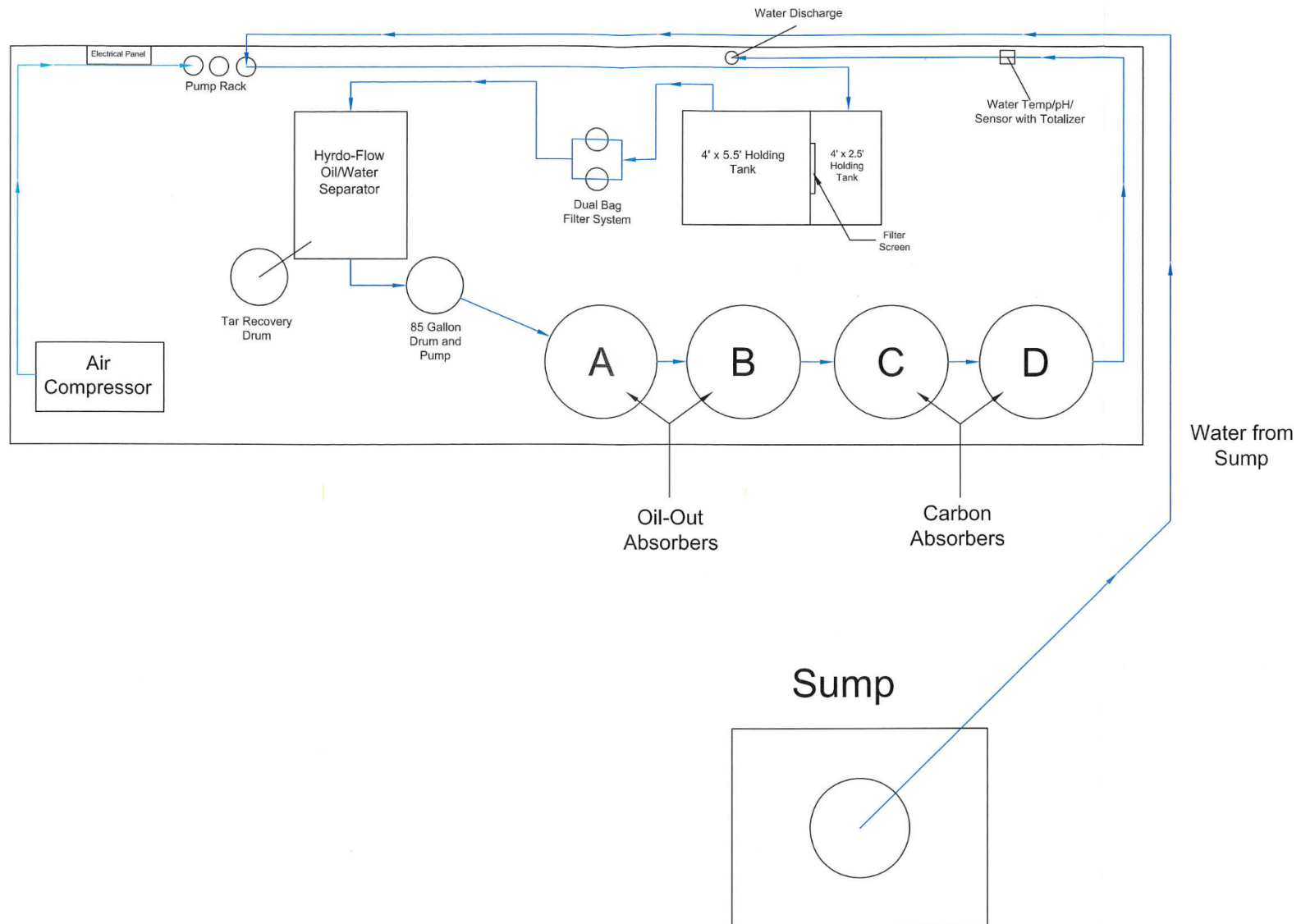
Figure 2. Treatment Process
