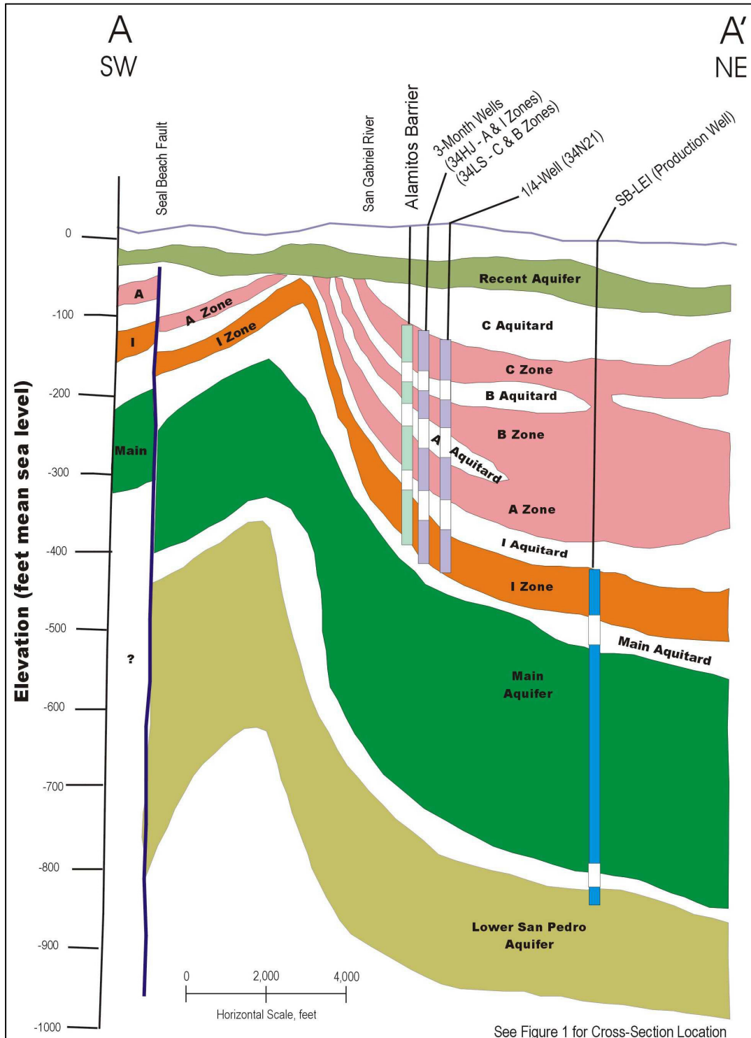
Figure P2 – Geologic Cross-Section A-A'
