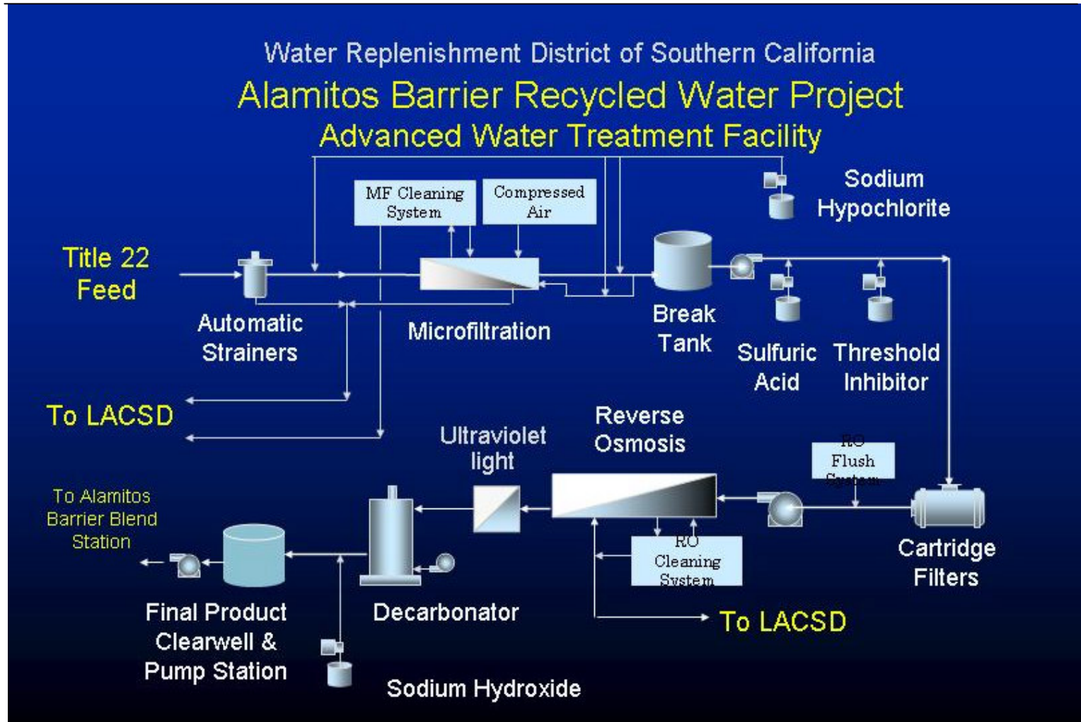
Figure P4 – Schematic of Treatment Process for Advanced Wastewater Treatment Facility
