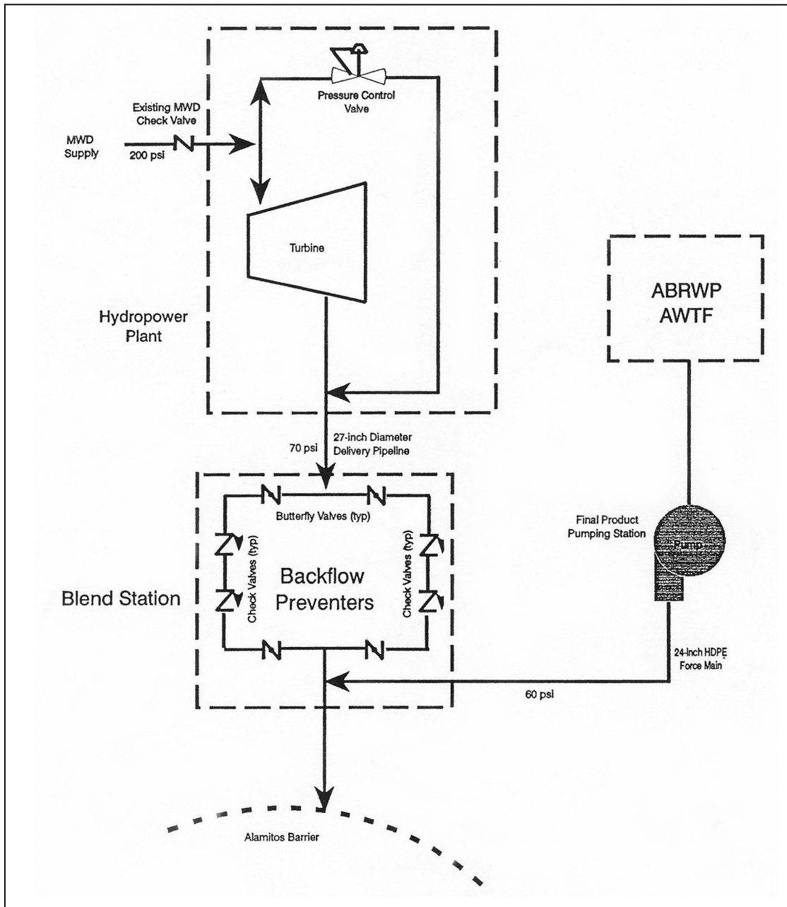
Figure P5 – Alamitos Barrier Water Supply and Blend Station Schematic Diagram
