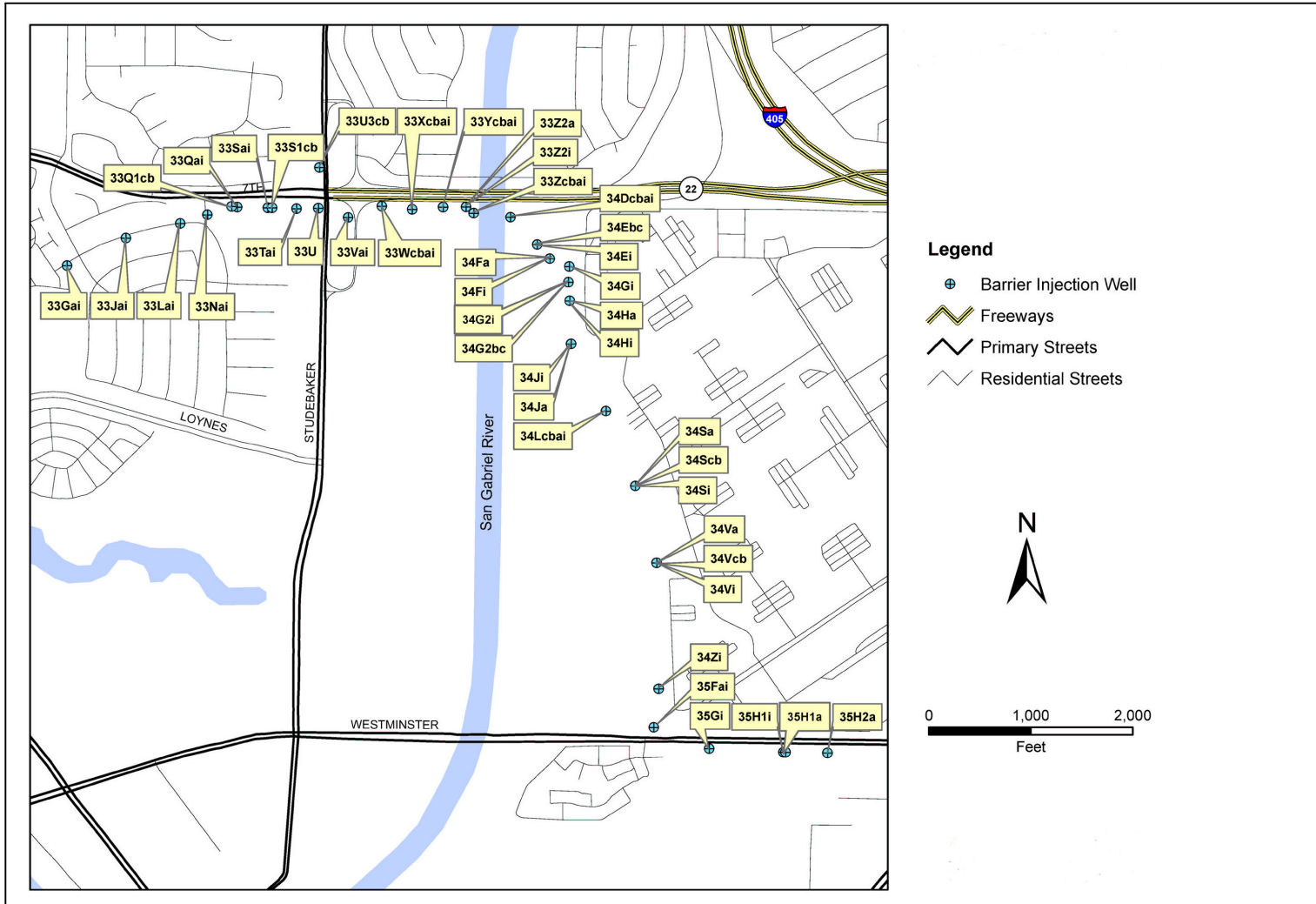
Figure P6 – Injection Well Locations of Alamitos Barrier Recycled Water Project
