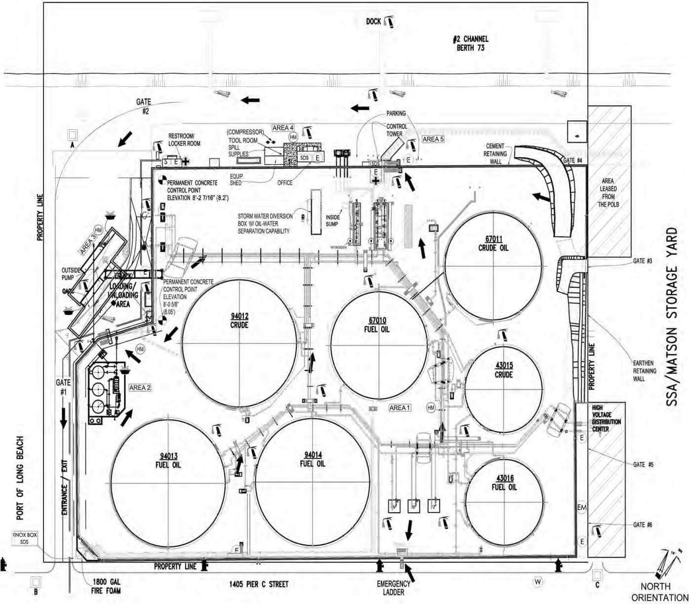
Figure 2. Site Plan
