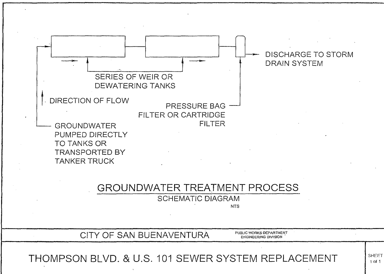
Figure 2-Treatment Schematic
