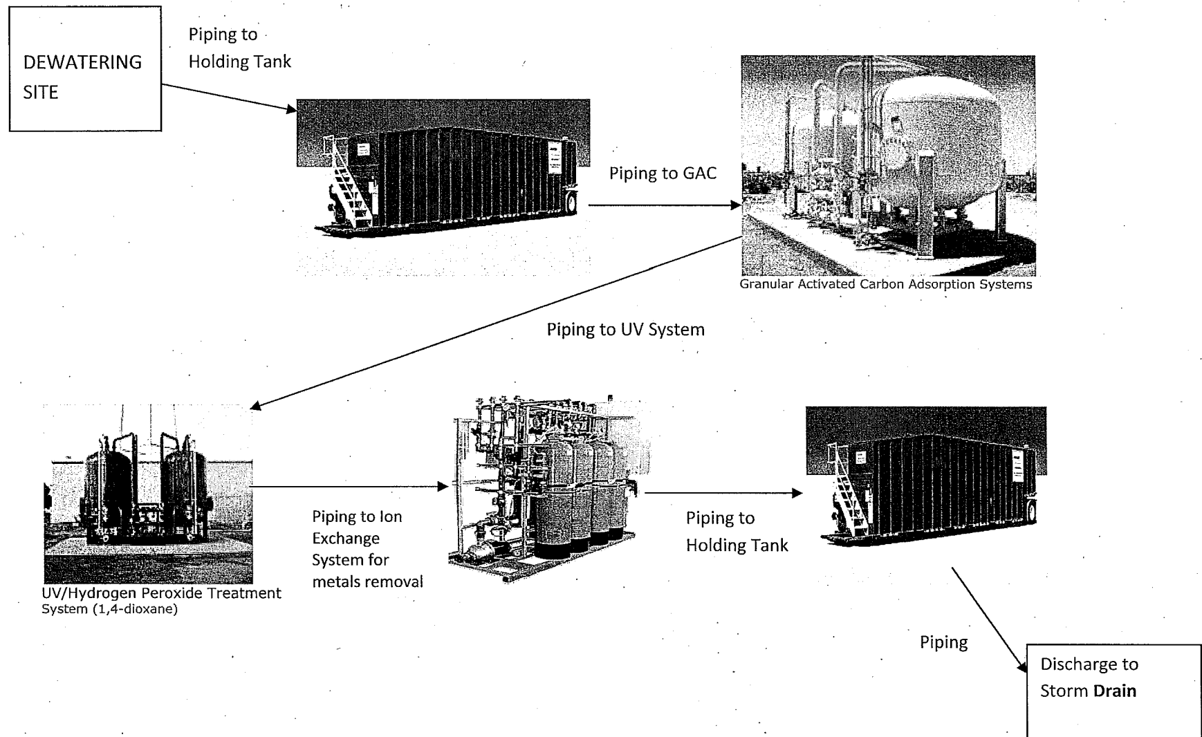
Figure 2 - Treatment Process
