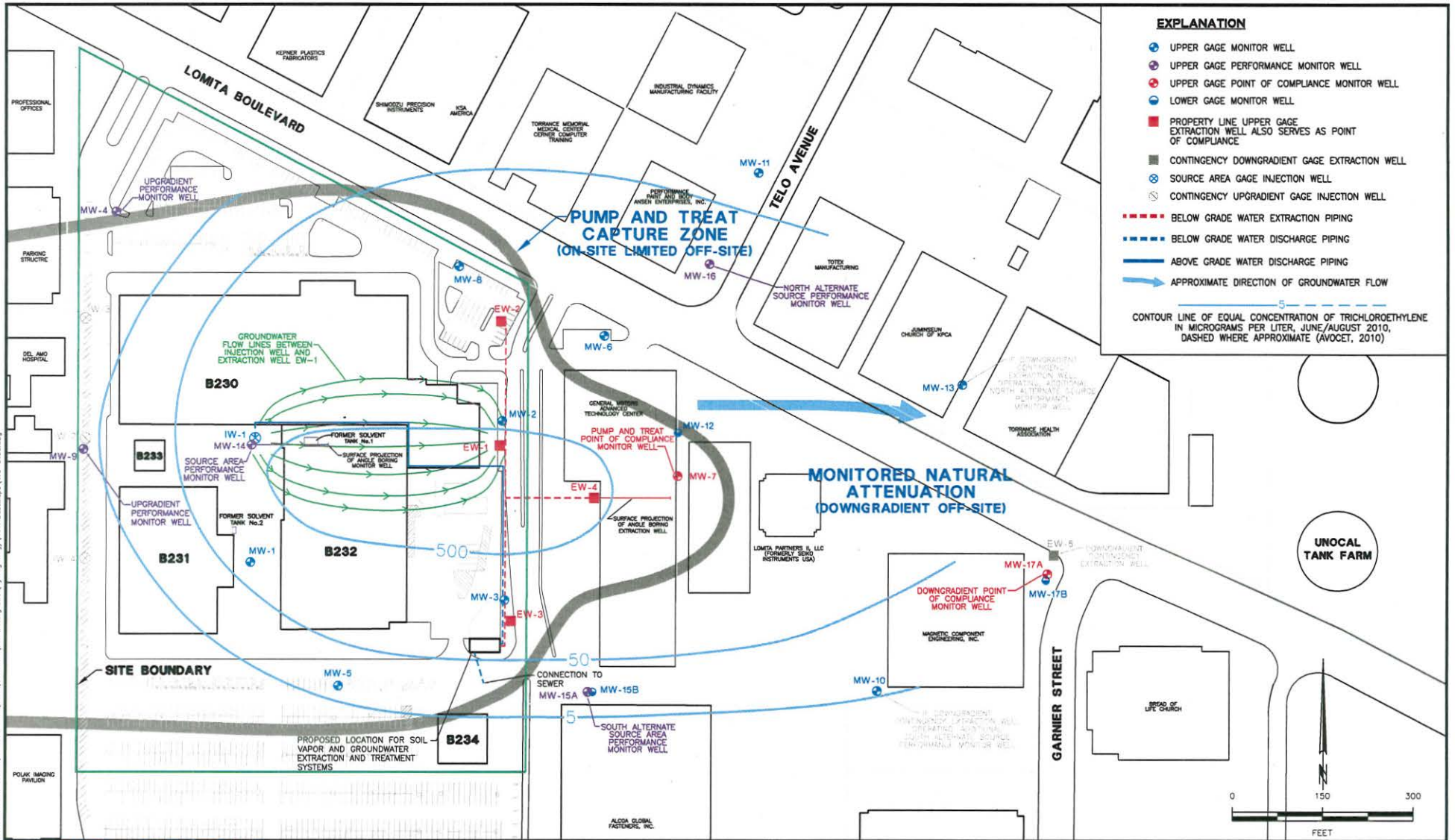
FIGURE 2. GROUNDWATER CORRECTIVE MEASURE
