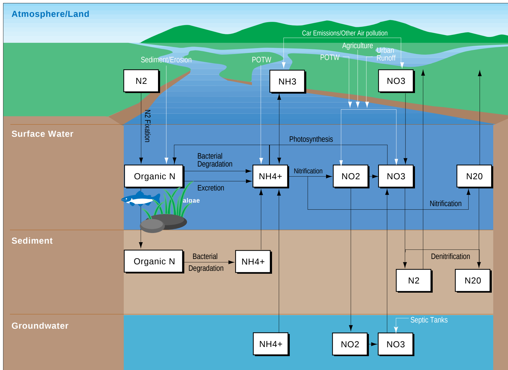
Figure 1-6. Conceptual Model of the Nitrogen Cycle
