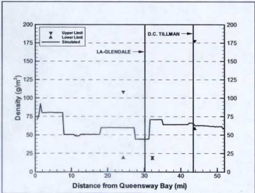
Figure 3-36. Simulated vs. Measured Attached Algae on the LA River for the 2000 Low Flow Period
