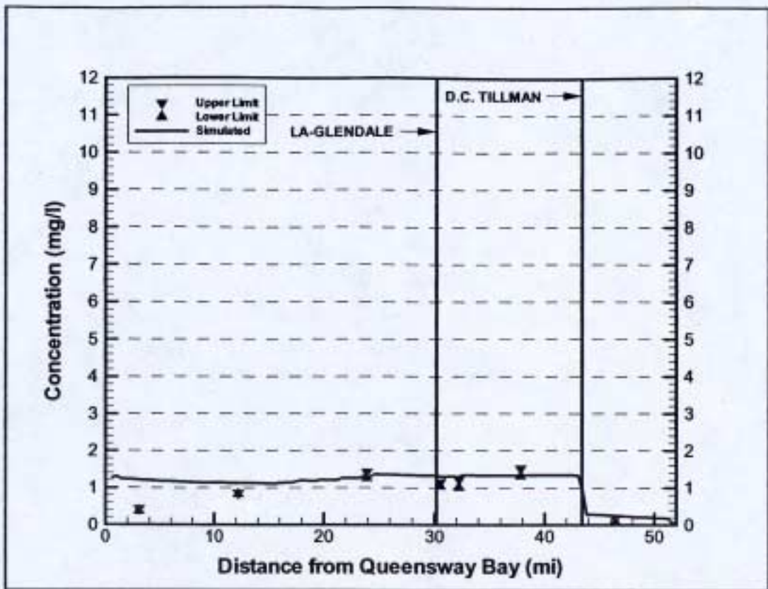
Figure 3-35. Simulated vs. Measured Total Phosphorous on the LA River for the 2000 Low Flow Period
