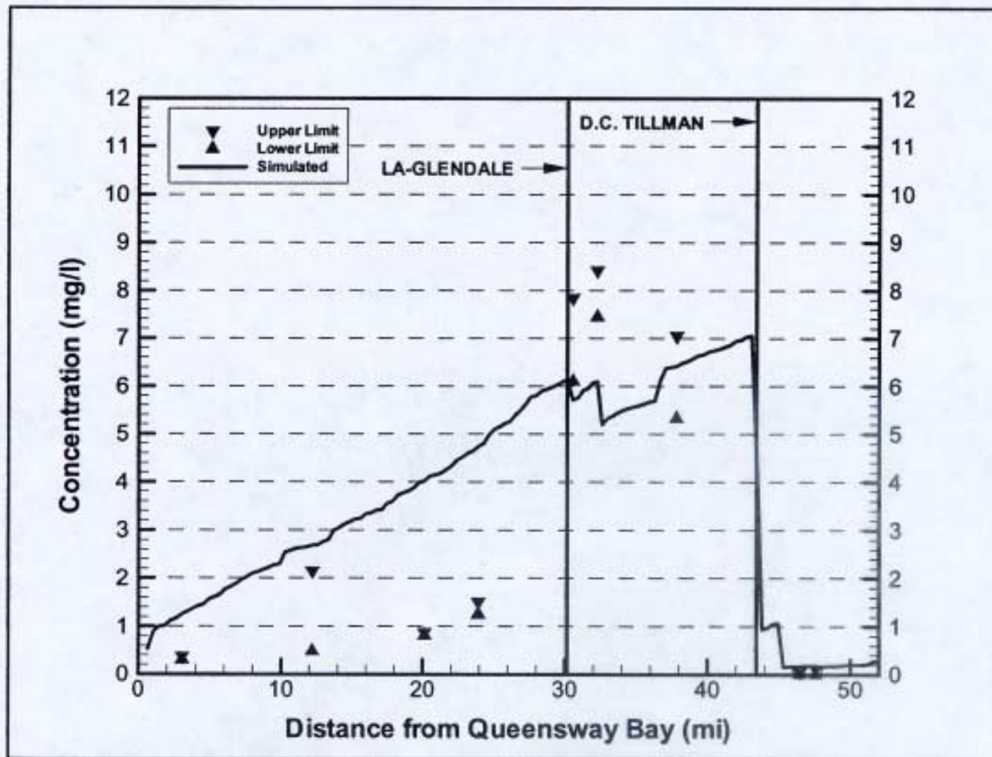
Figure 3-37. Simulated vs. Measured Ammonia on the LA River for the 2001 Low Flow Period
