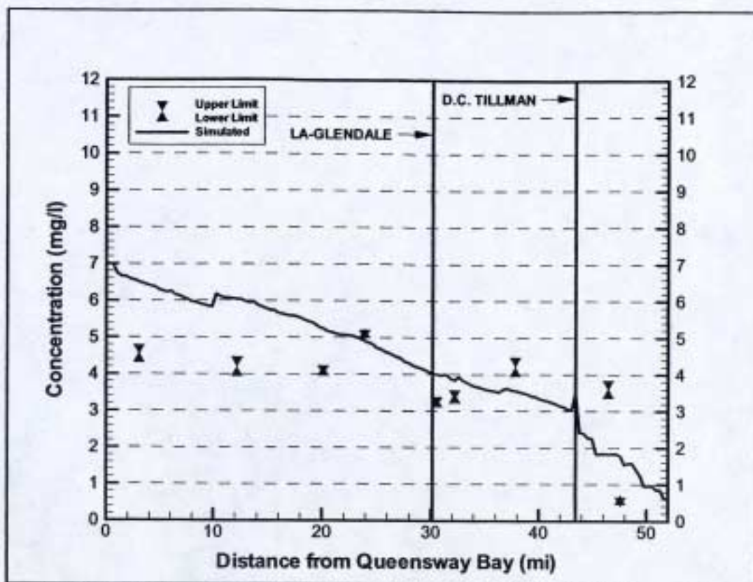
Figure 3-38. Simulated vs. Measured Nitrate+Nitrite on the LA River for the 2001 Low Flow Period
