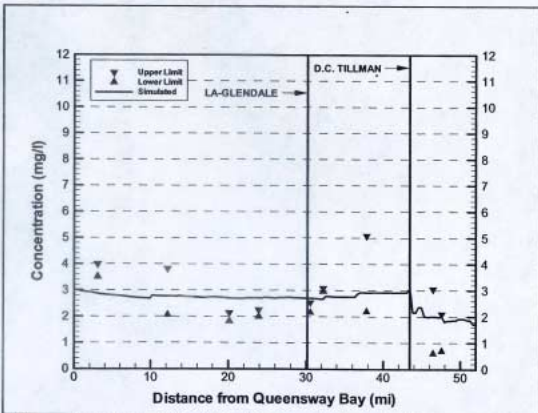
Figure 3-39. Simulated vs. Measured Organic Nitrogen on the LA River for the 2001 Low Flow Period
