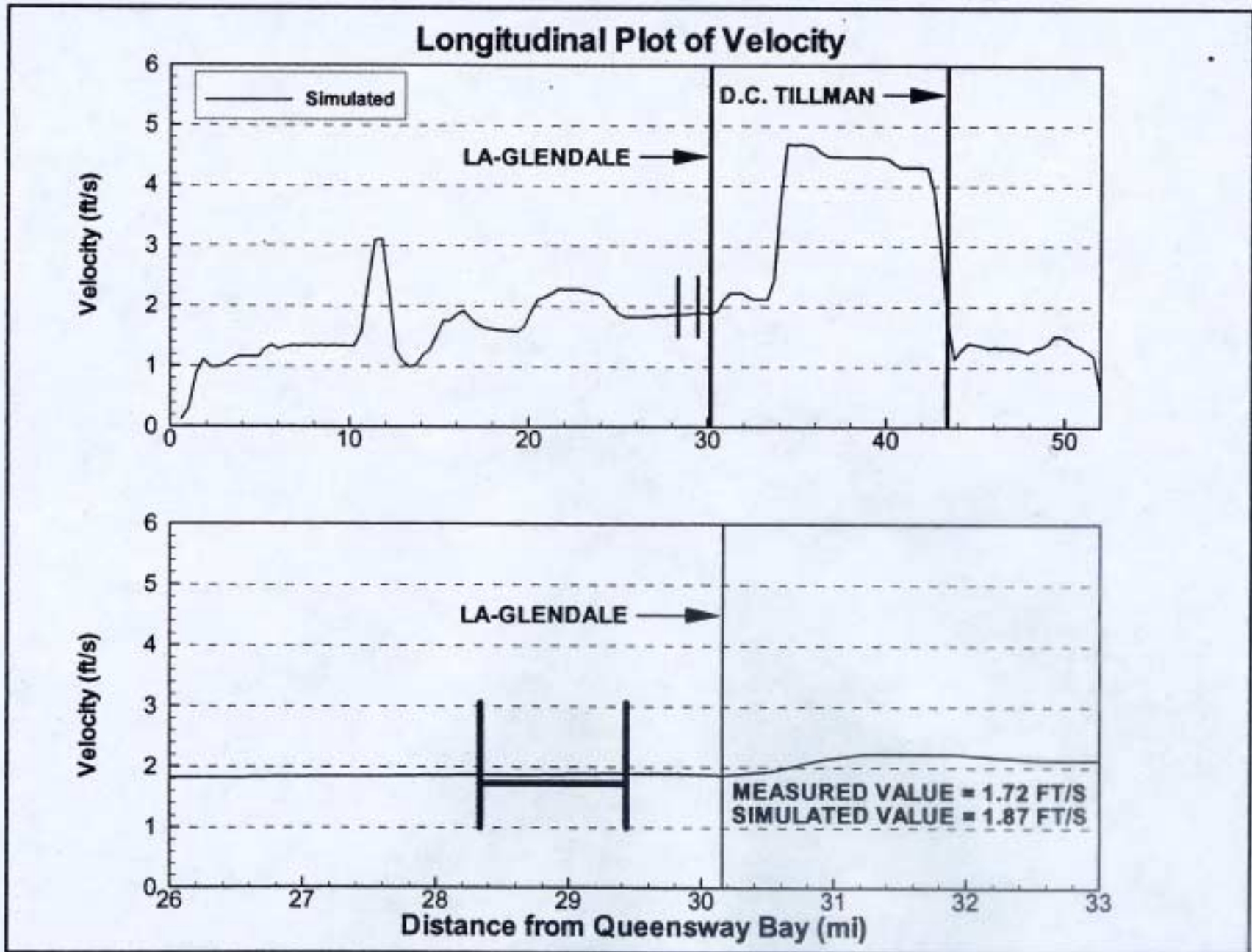
Figure 3-13. Simulated vs. Measured Velocity During 2000 Low Flow Period
