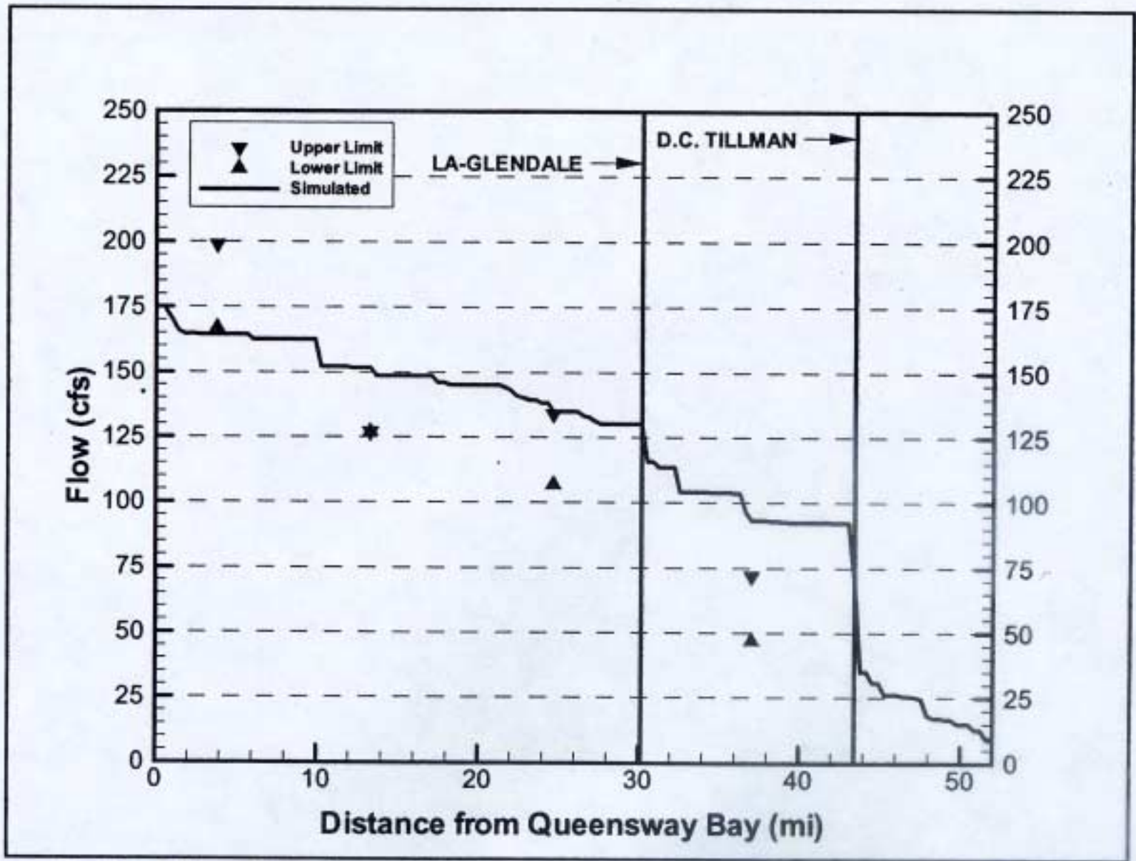
Figure 3-14. Simulated vs. Measured Flow During 2001 Low Flow Period
