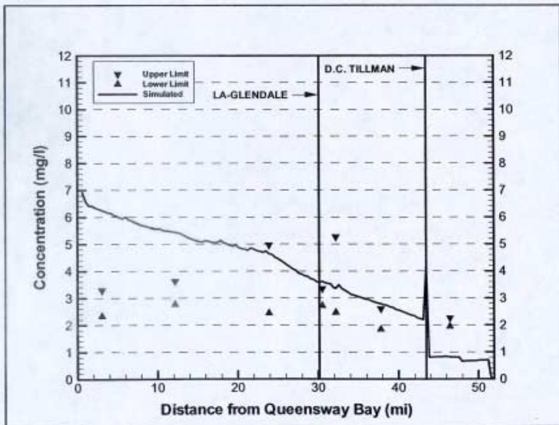
Figure 3-32. Simulated vs. Measured Nitrate+Nitrite on the LA River for the 2000 Low Flow Period
