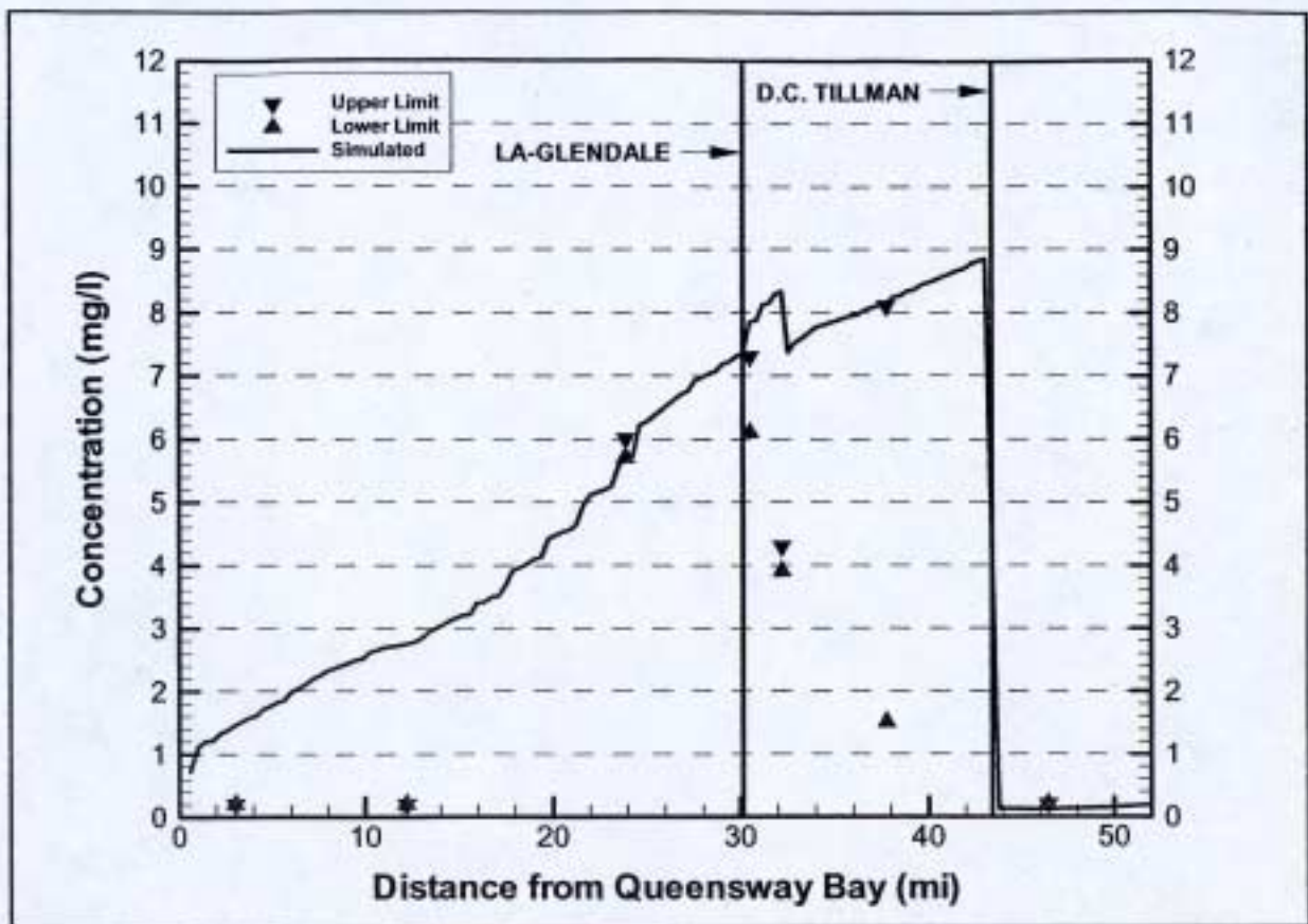
Figure 3-31. Simulated vs. Measured Ammonia on the LA River for the 2000 Low Flow Period
