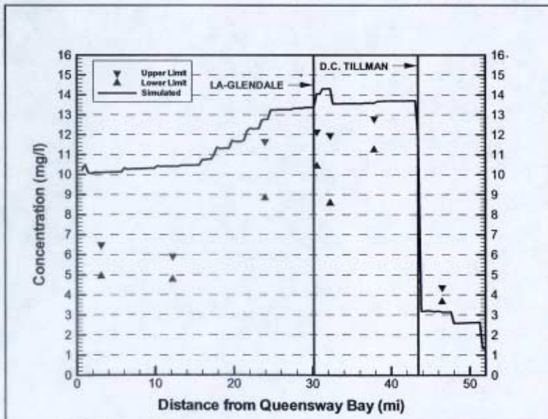
Figure 3-34. Simulated vs. Measured Total Nitrogen on the LA River for the 2000 Low Flow Period
