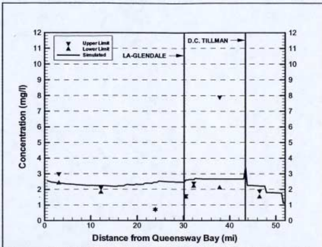
Figure 3-33. Simulated vs. Measured Organic Nitrogen on the LA River for the 2000 Low Flow Period
