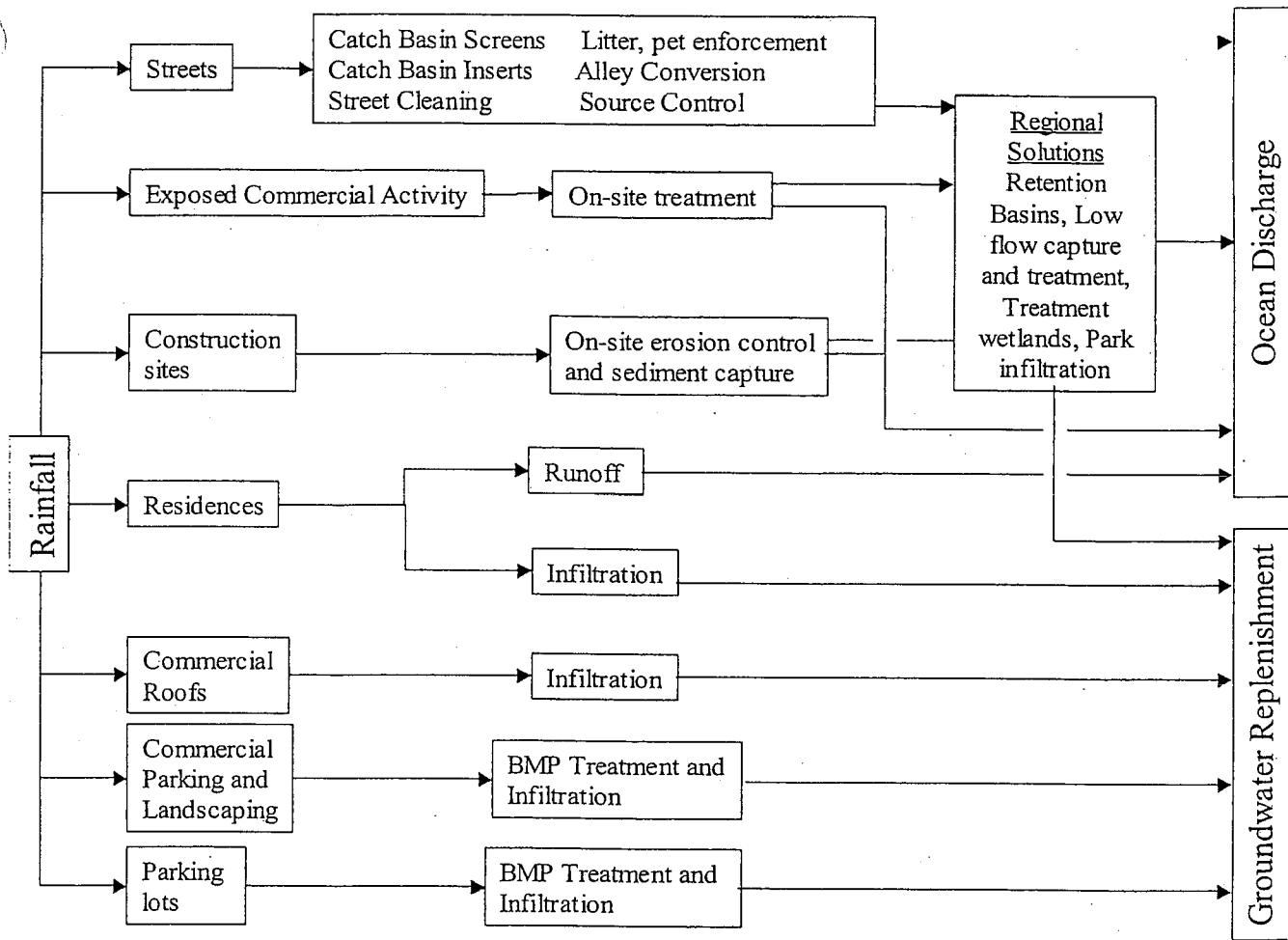
Figure 1. Stormwater quality control solutions for Southern California
