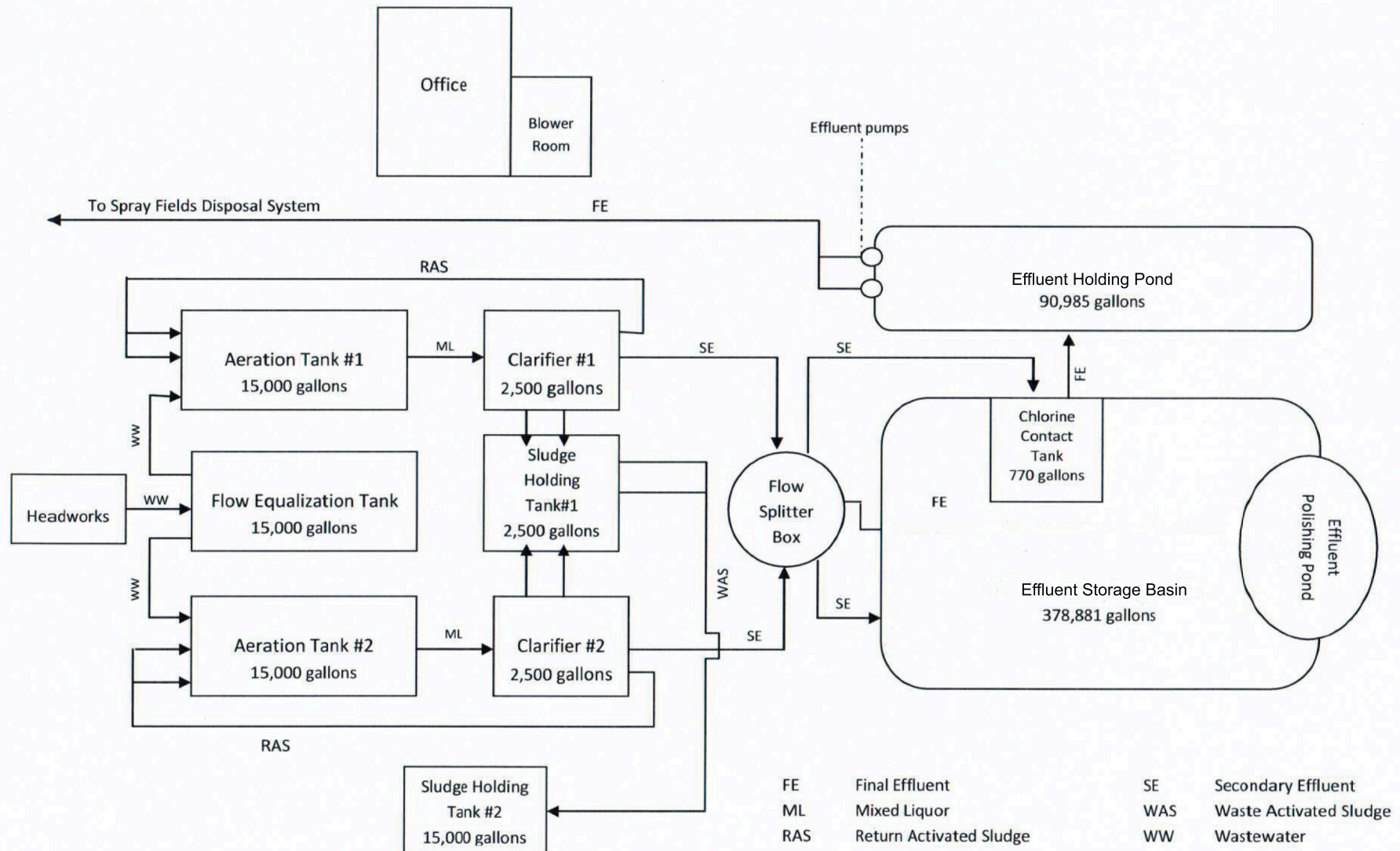
Figure 3: Existing Process Schematic
