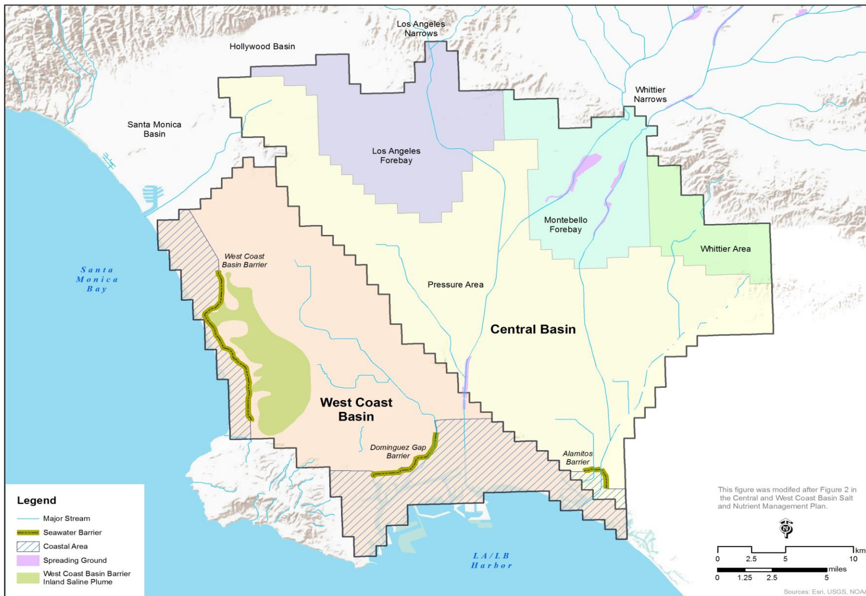
Figure 8.1-1. Central Basin and West Coast Basin Subareas and Coastal Areas (modeled).
